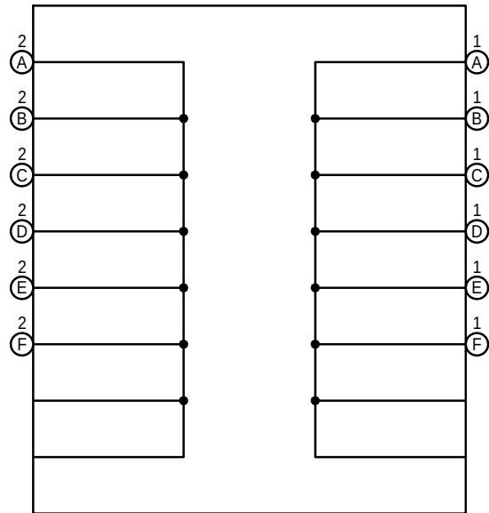
K146(A), K147(B), K148(C), K149(D), K150(E), K151(F) No. 10 CAN Junction Connector
