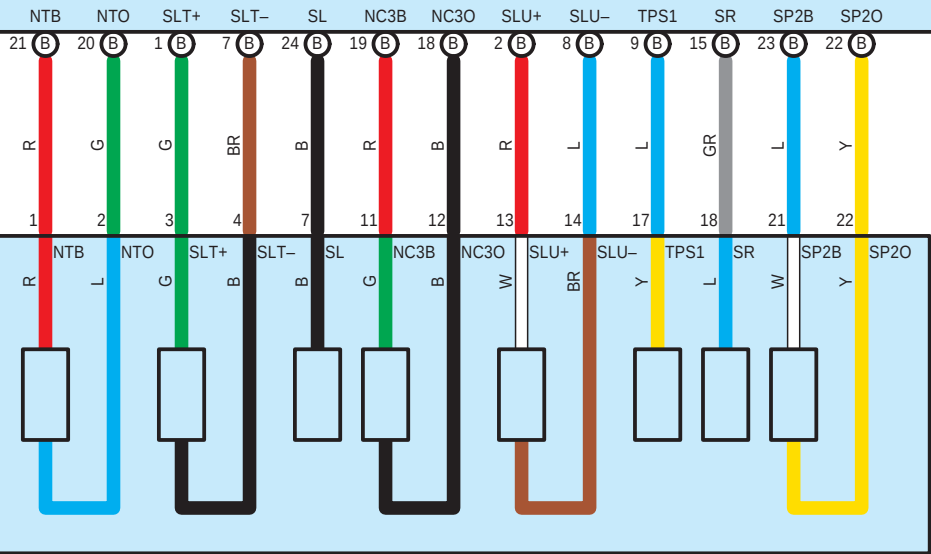
F73 ECT Solenoid (Transmission Wire)
