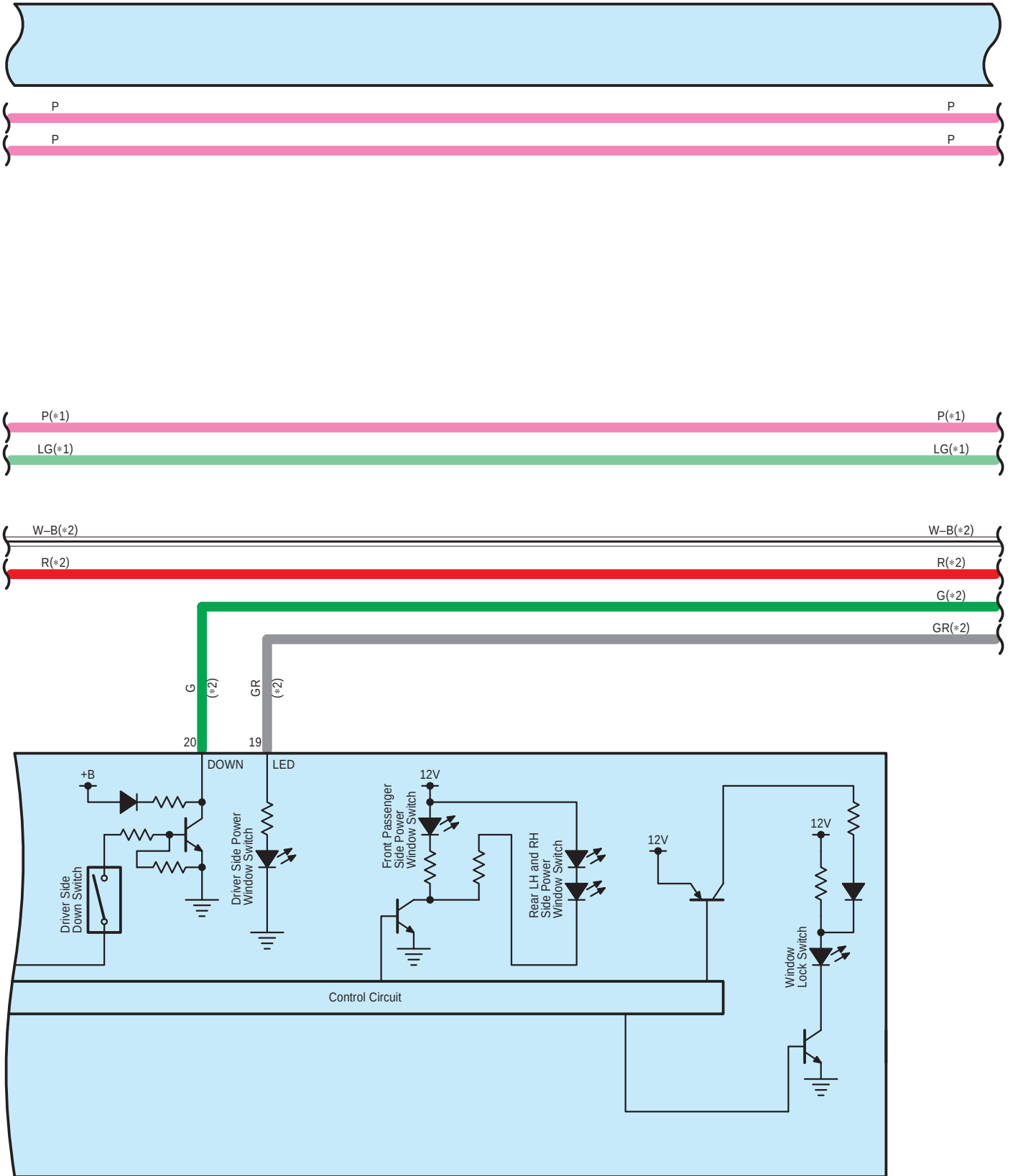
N12 Multiplex Network Master Switch Assembly
