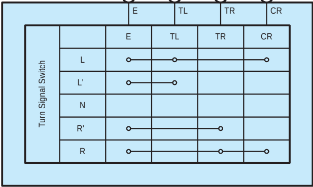
K23(A) Headlight Dimmer Switch Assembly
