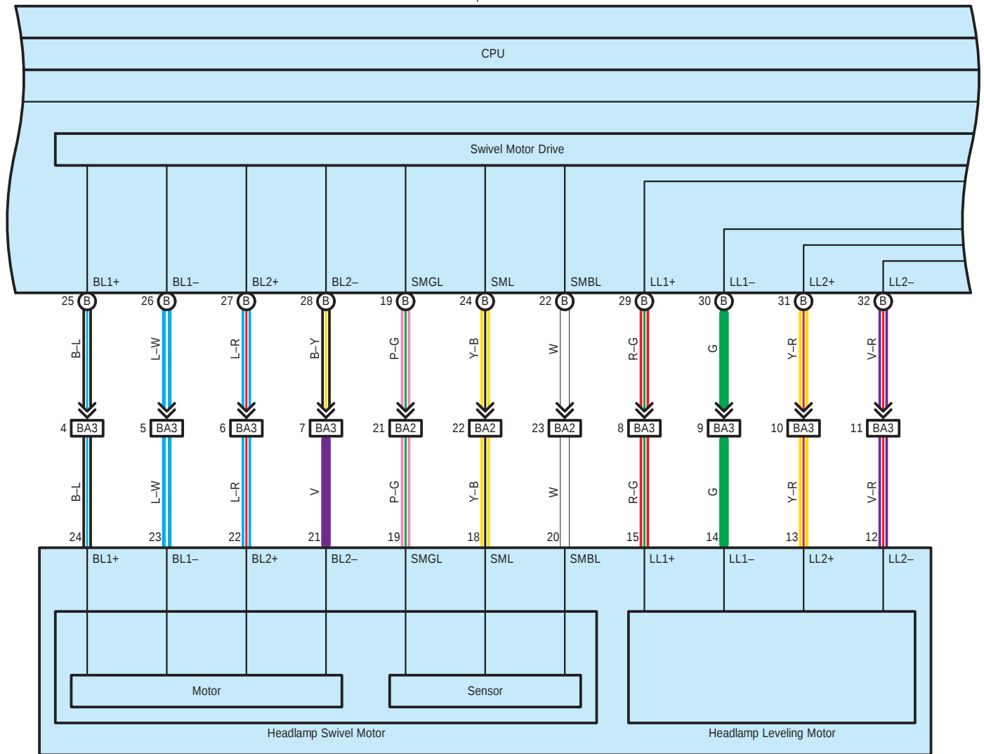
B12 Headlamp Assembly (LH)
