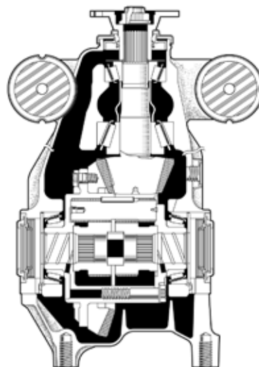
F20TX (TORSEN* LSD)
