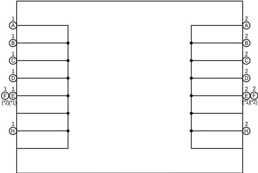
X100(A), X101(B), X102(C), X103(D), X104(E), X105(F), X107(H) No. 13 CAN Junction Connector
