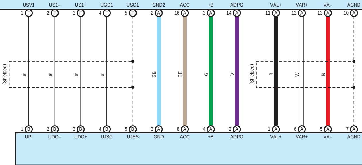
P77(A), P102(B) No. 1 Stereo Jack Adapter Assembly
