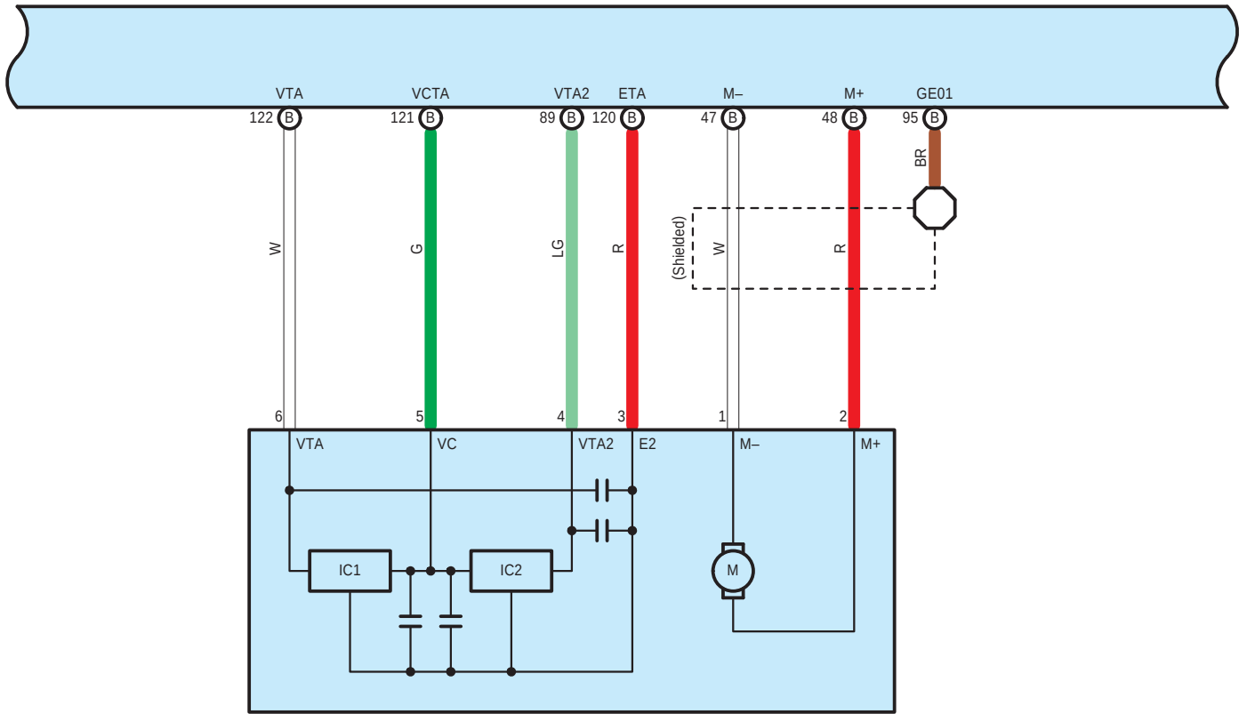
G10 Throttle Body with Motor Assembly
