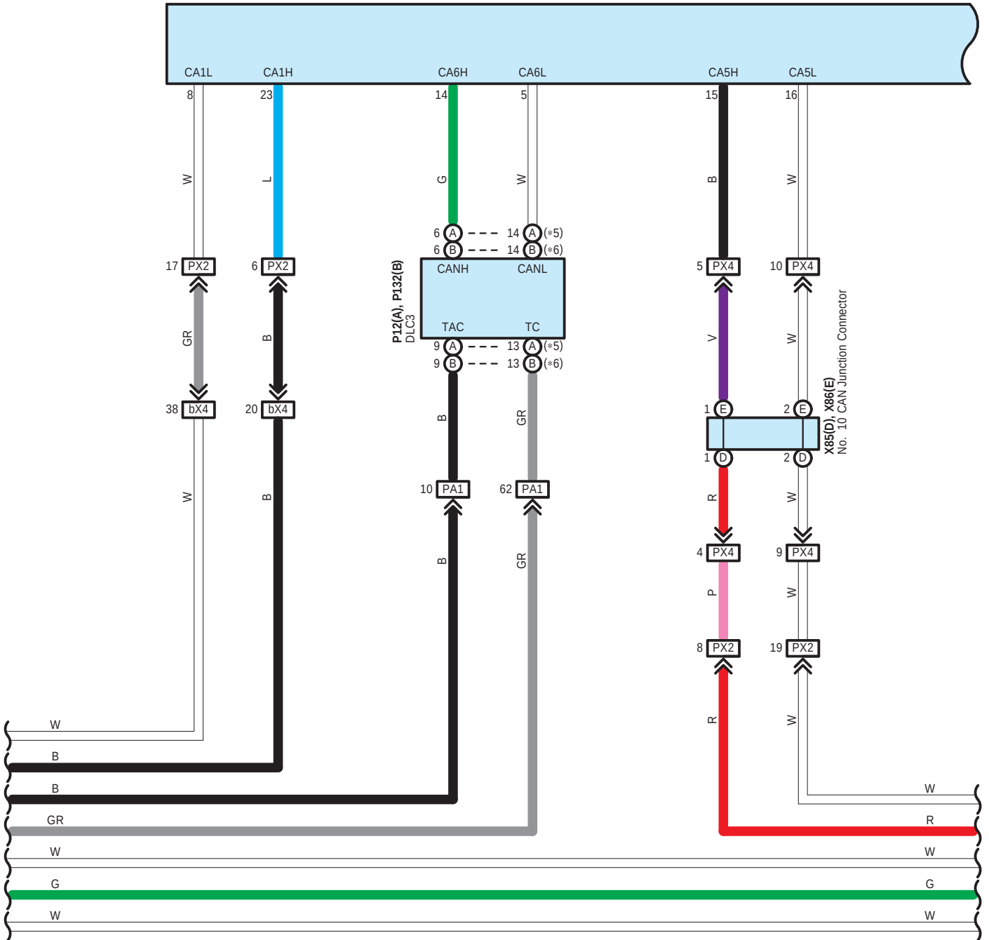
P59 Network Gateway ECU
