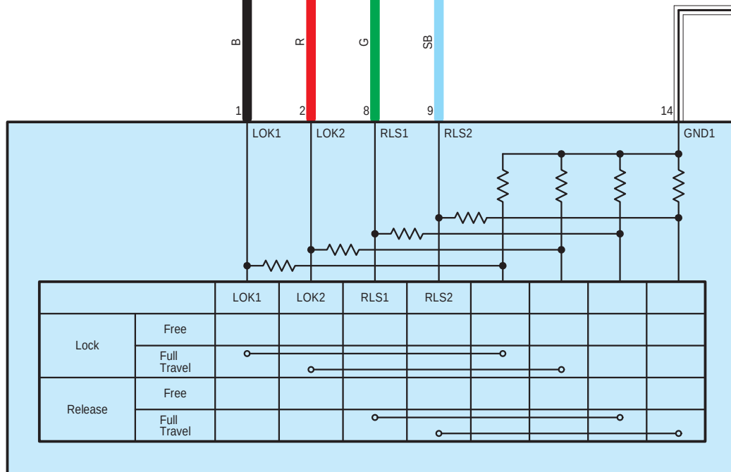
P36 Electric Parking Brake Switch Assembly
