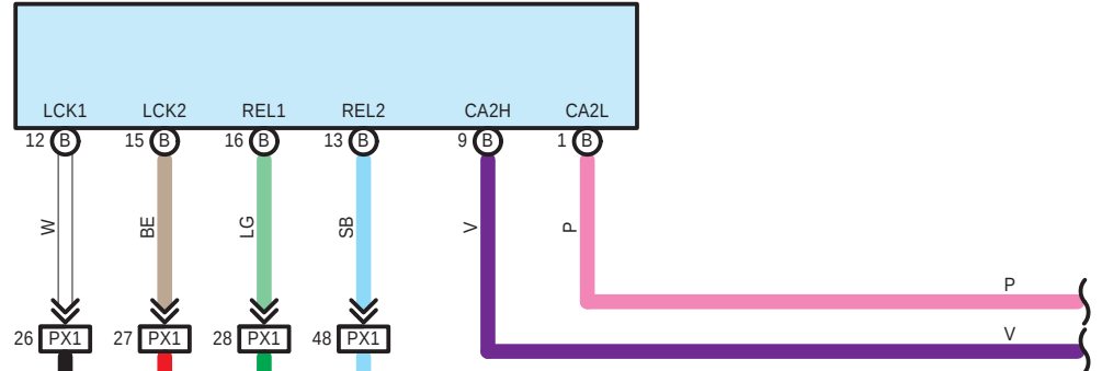
X67(B) Parking Brake ECU Assembly
