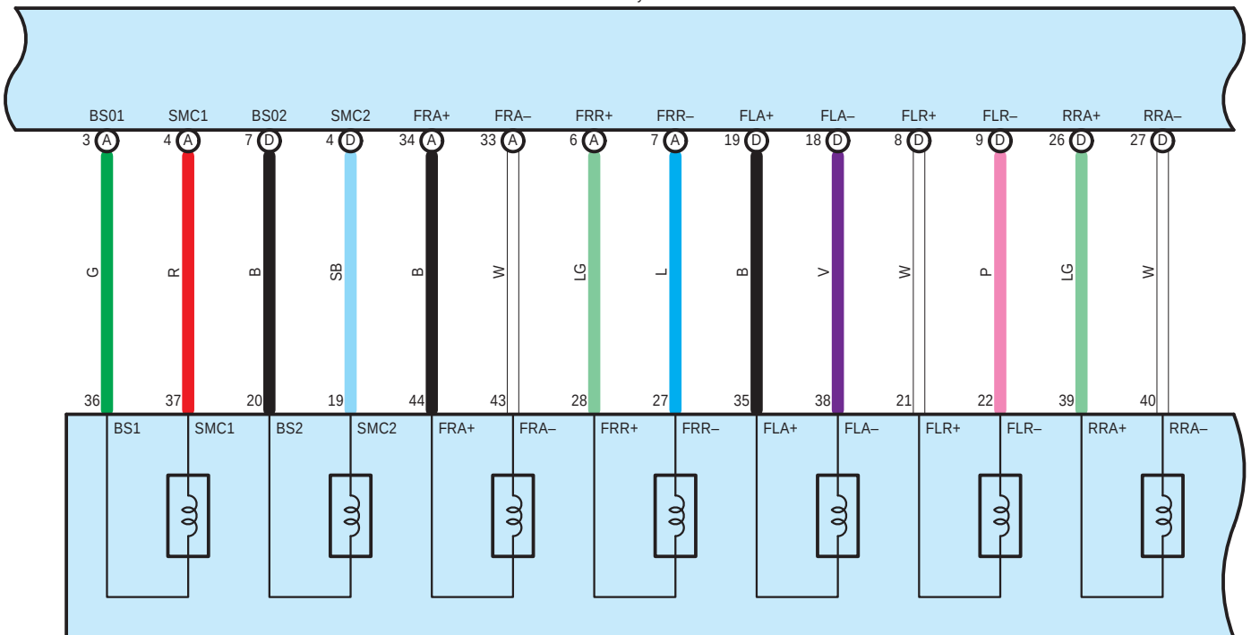
A7 Brake Actuator Assembly
