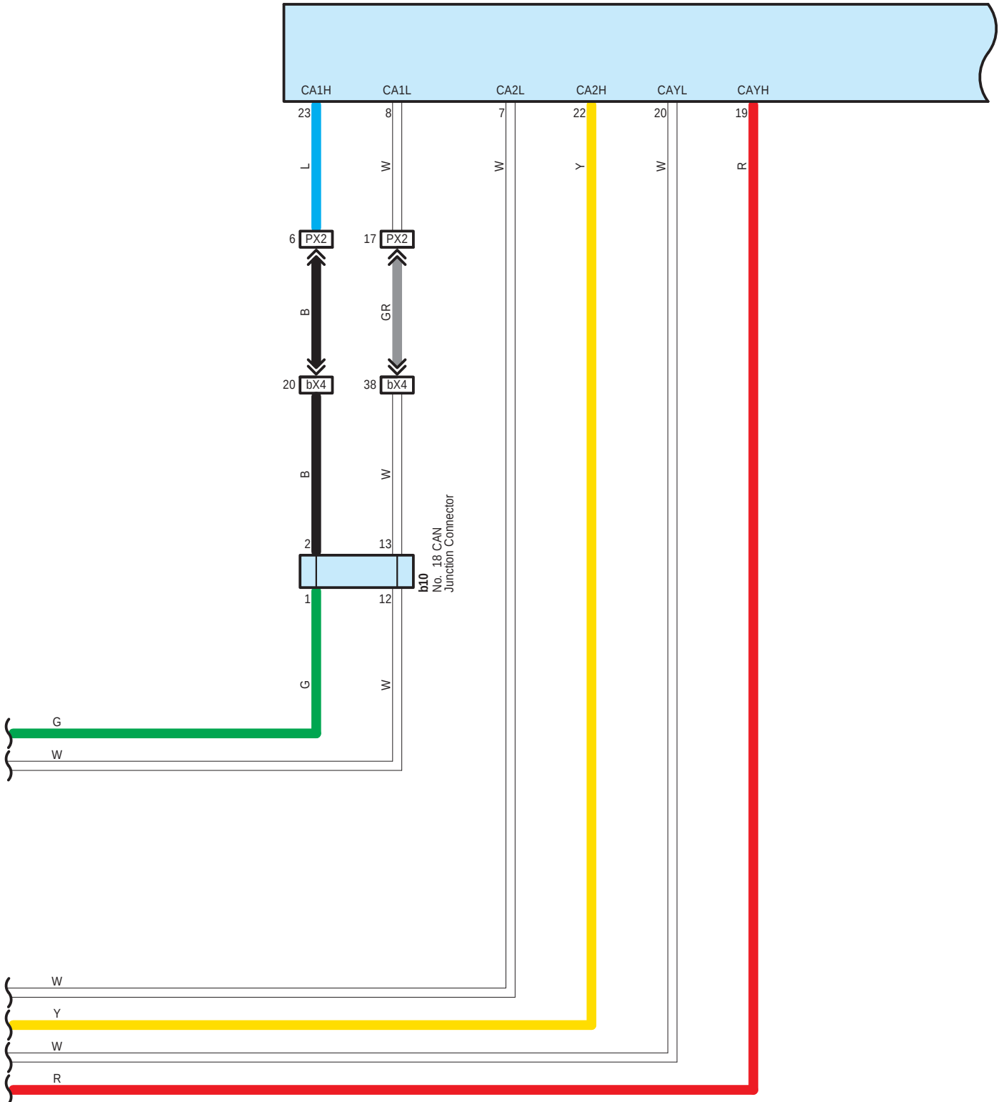
P59 Network Gateway ECU
