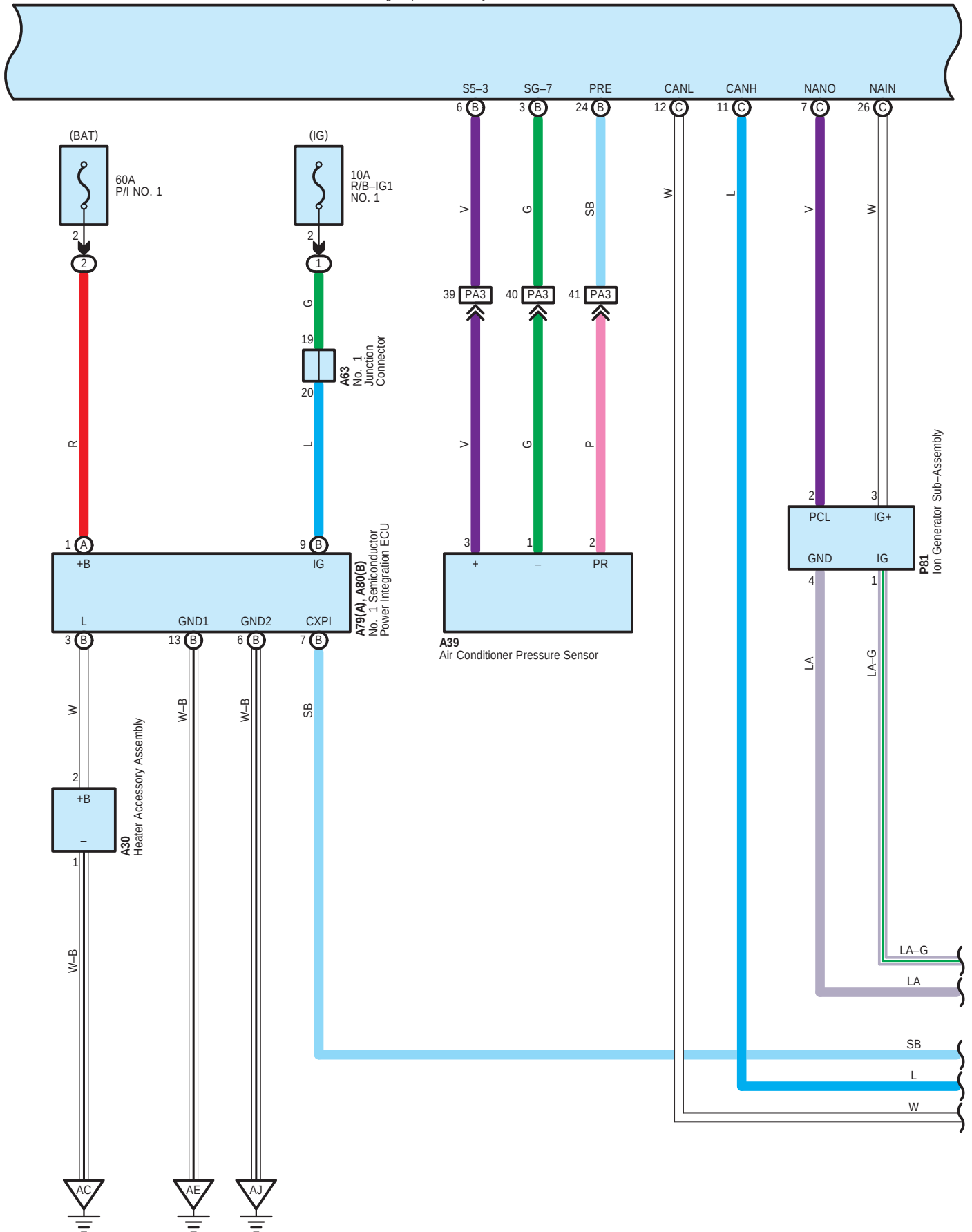
P57(B), P58(C), z1(D) Air Conditioning Amplifier Assembly
