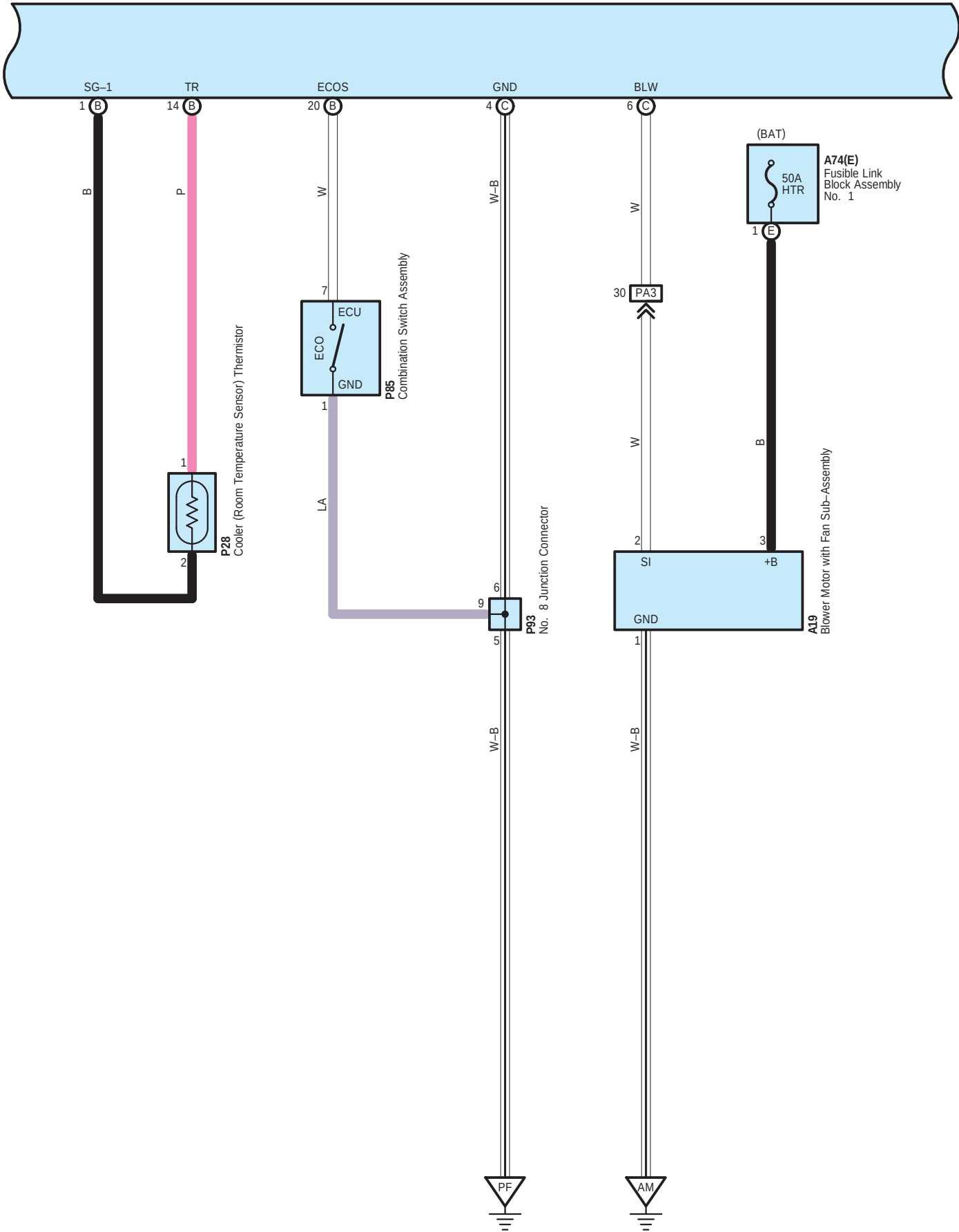
P57(B), P58(C), z1(D) Air Conditioning Amplifier Assembly
