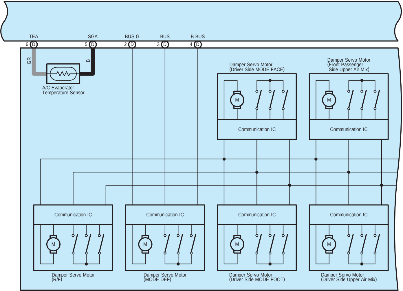
z1(D) Air Conditioning Harness Assembly
