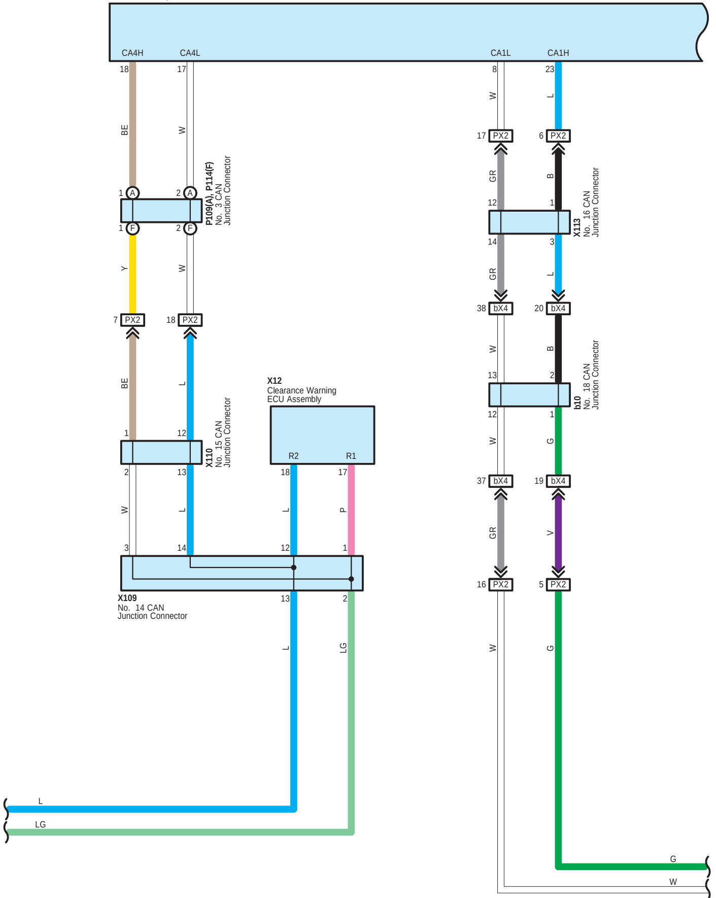
P59 Network Gateway ECU
