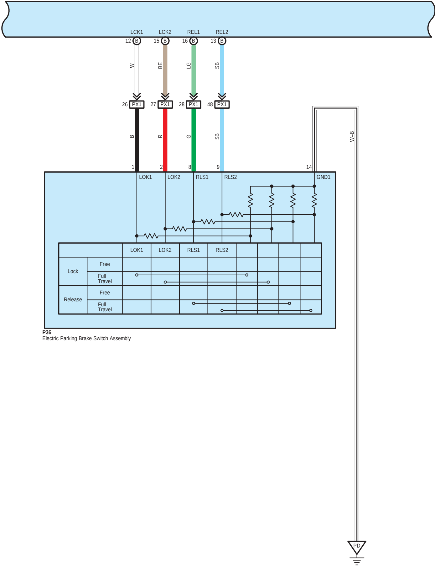
X66(A), X67(B) Parking Brake ECU Assembly
