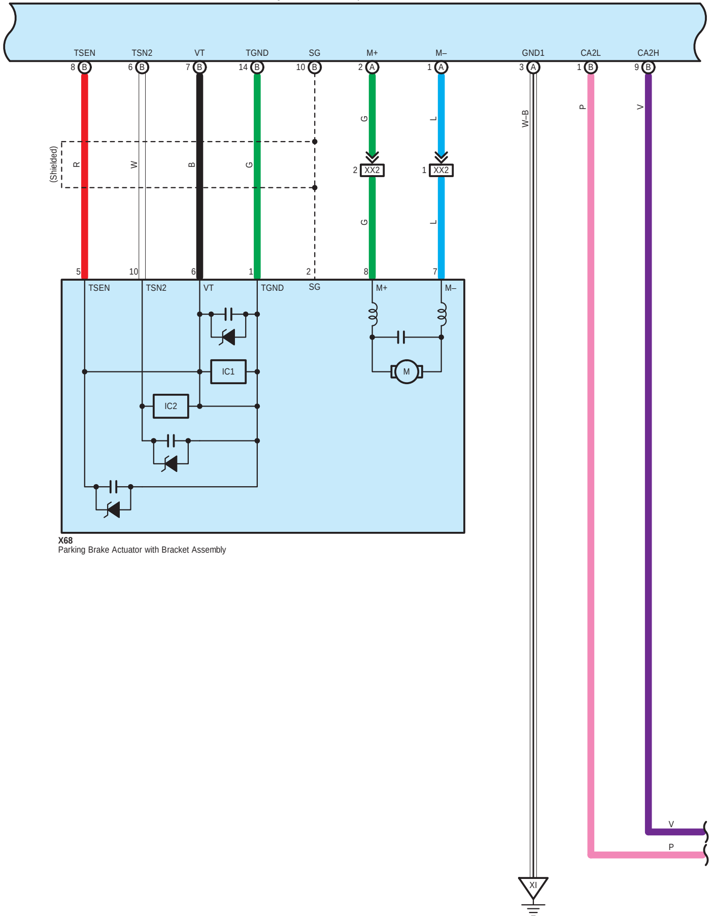
X66(A), X67(B) Parking Brake ECU Assembly
