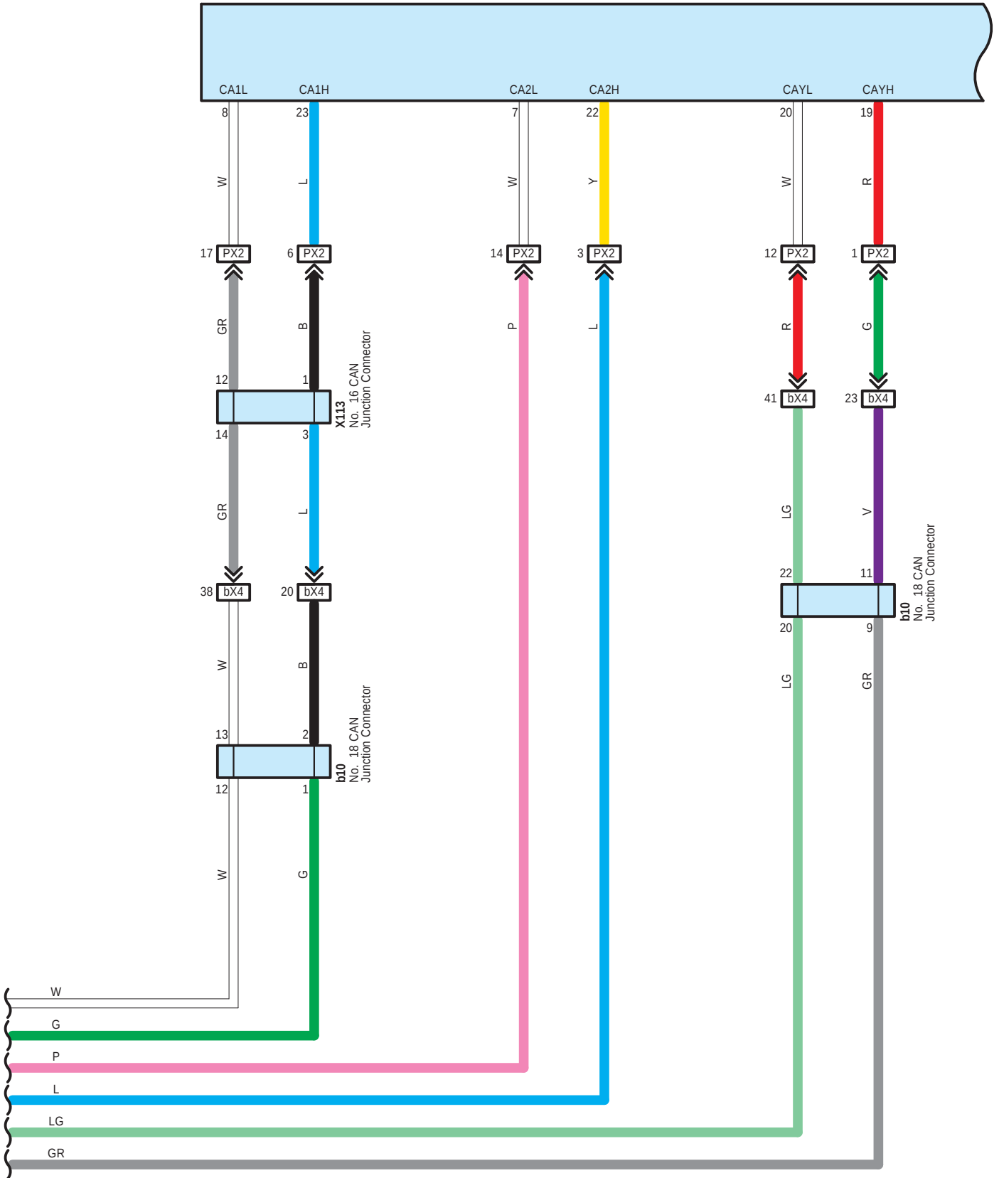
P59 Network Gateway ECU
