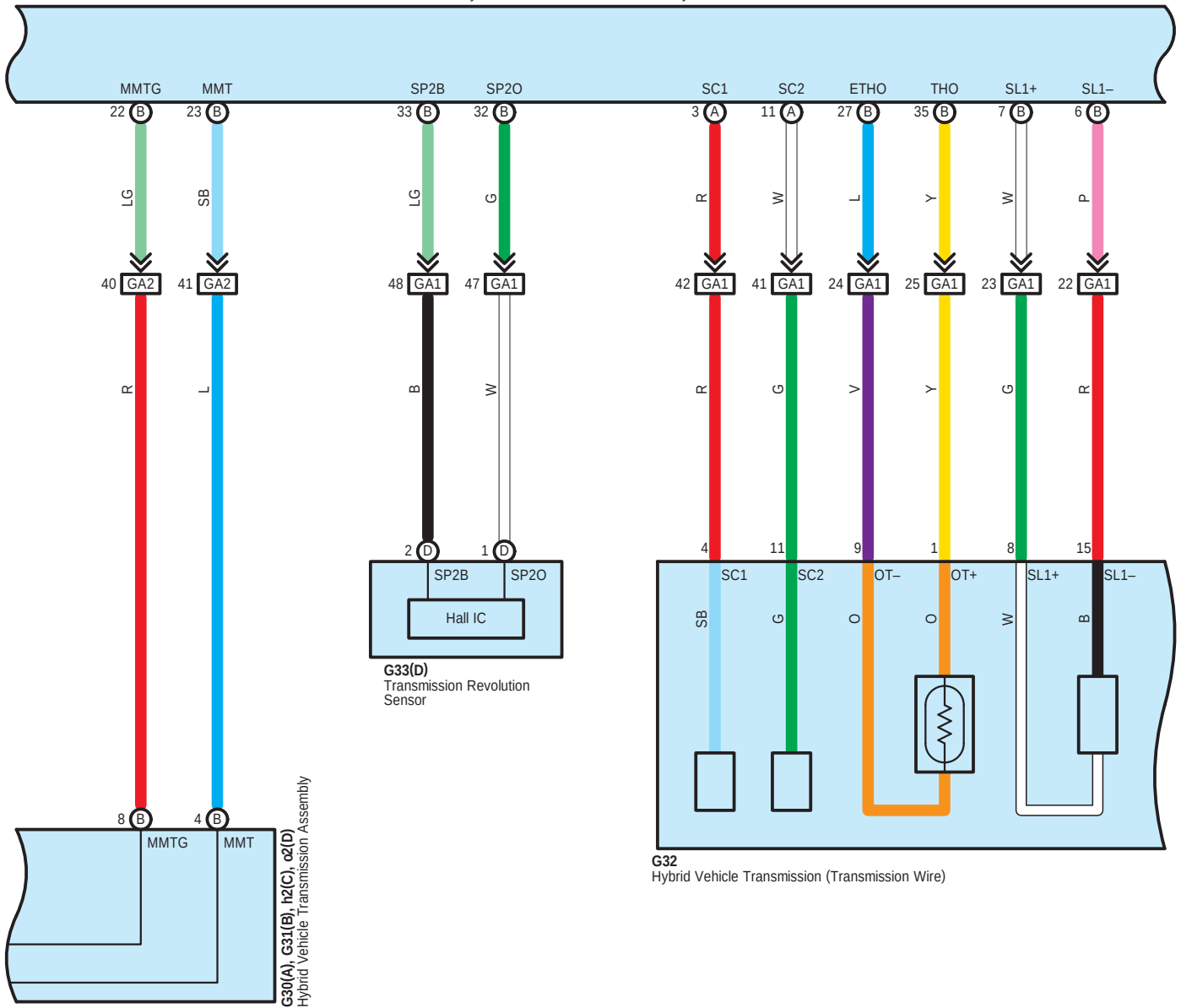
A21(A), A22(B), P64(C), P65(D) Hybrid Vehicle Control ECU Assembly
