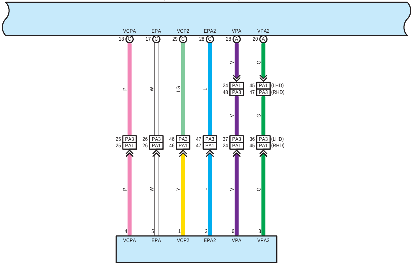
A1 Accelerator Pedal Sensor Assembly
