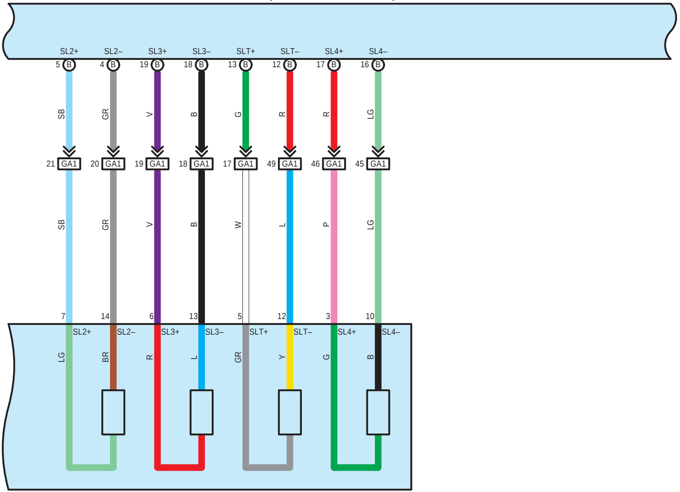
G32 Hybrid Vehicle Transmission (Transmission Wire)
