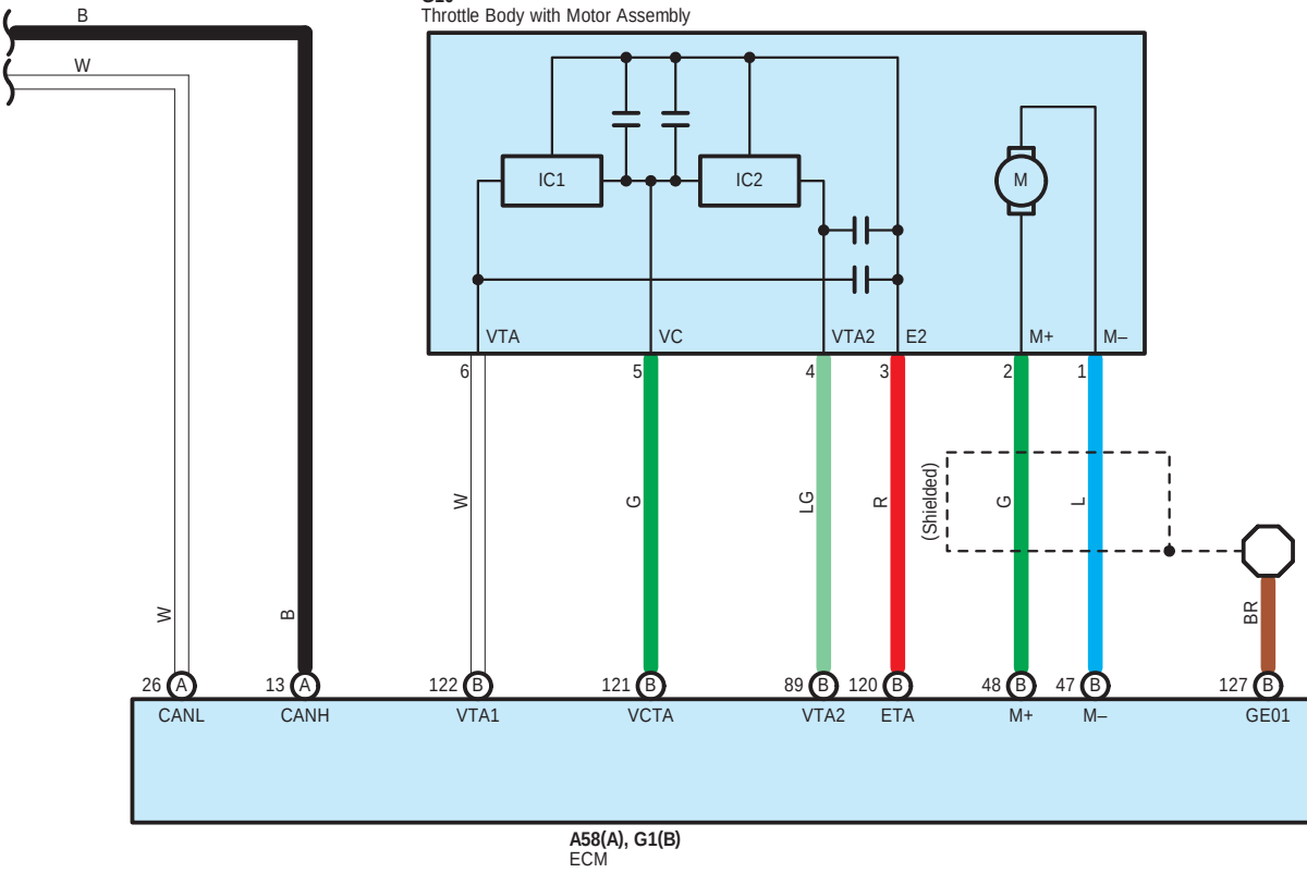
G10 Throttle Body with Motor Assembly
