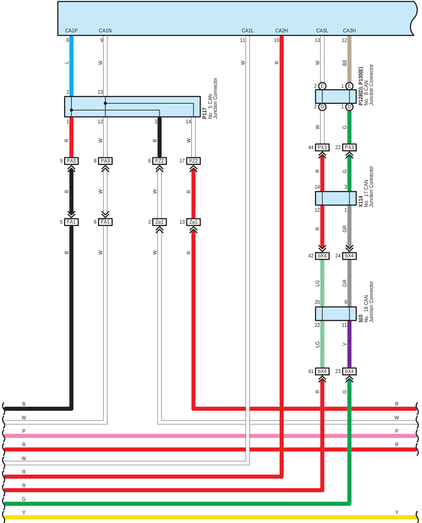
P62 Driving Support ECU Assembly
