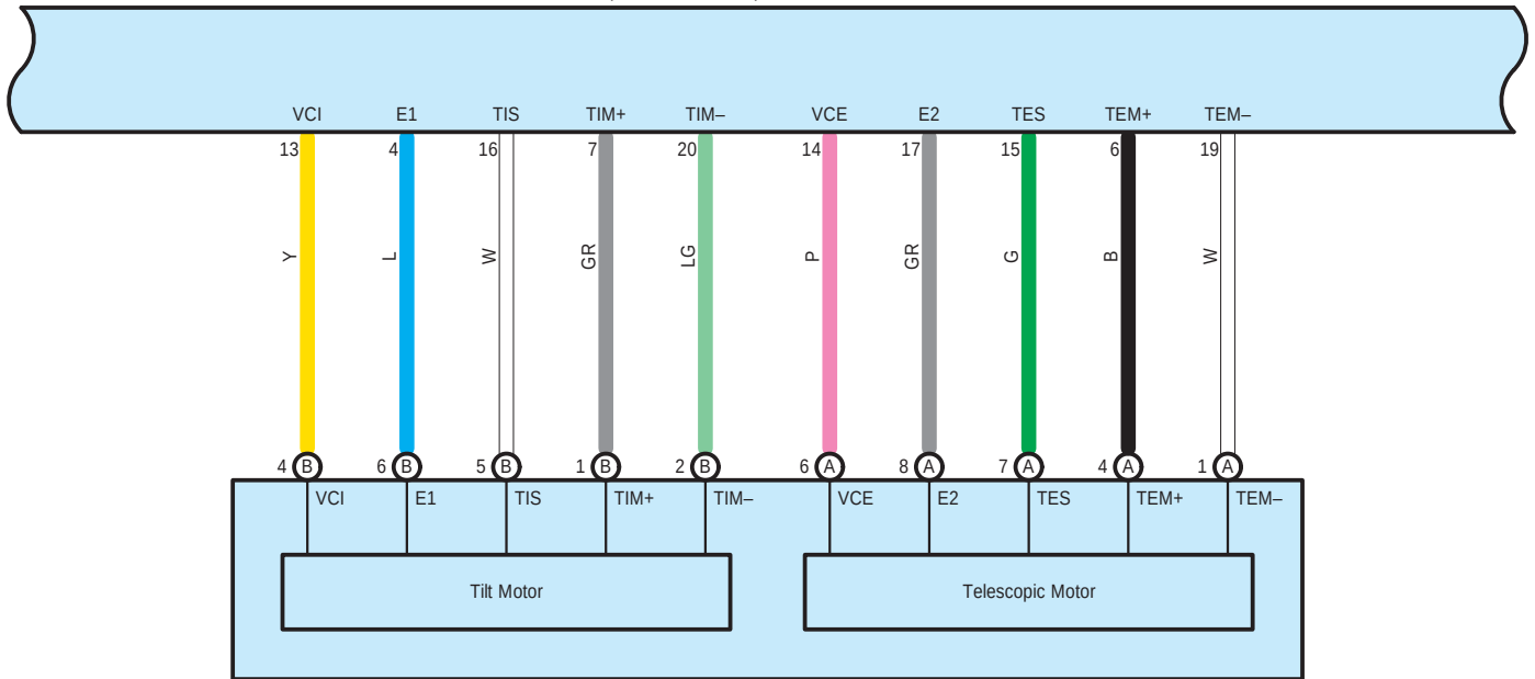
P15(A), P23(B) Steering Column Assembly
