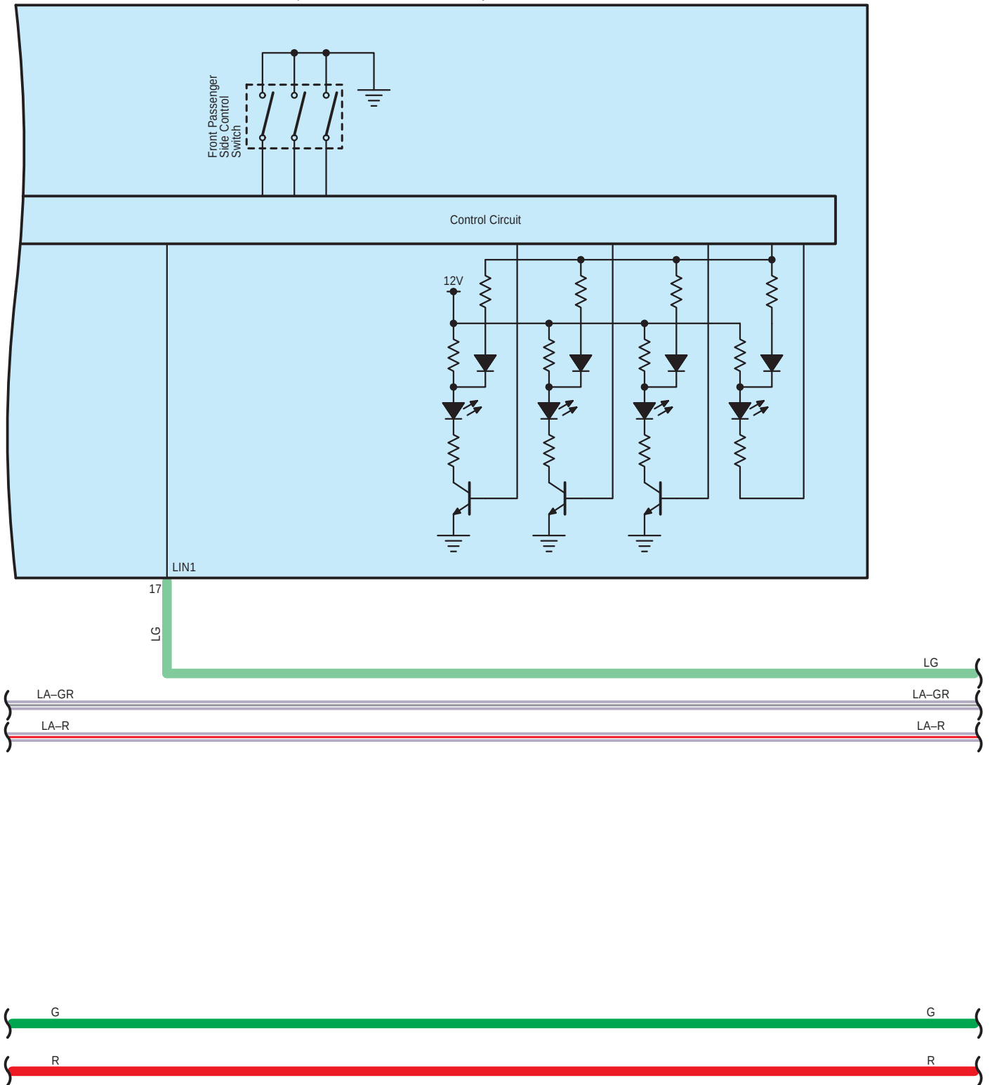
T2 Multiplex Network Master Switch Assembly
