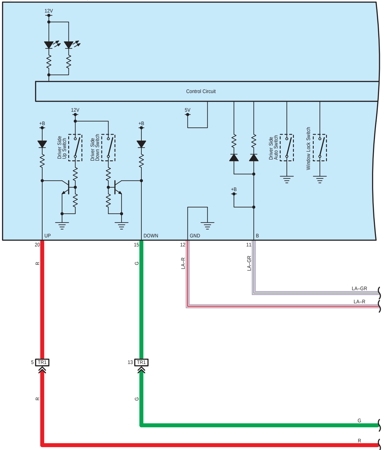
T2 Multiplex Network Master Switch Assembly
