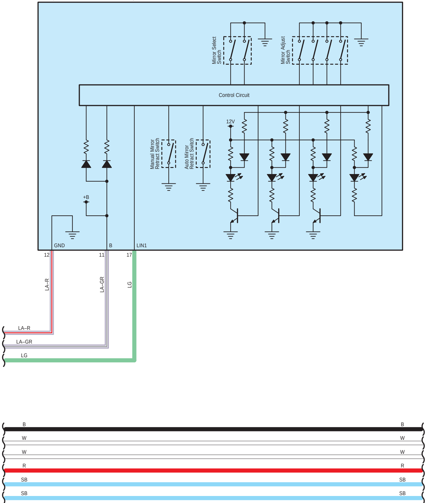
T2 Multiplex Network Master Switch Assembly
