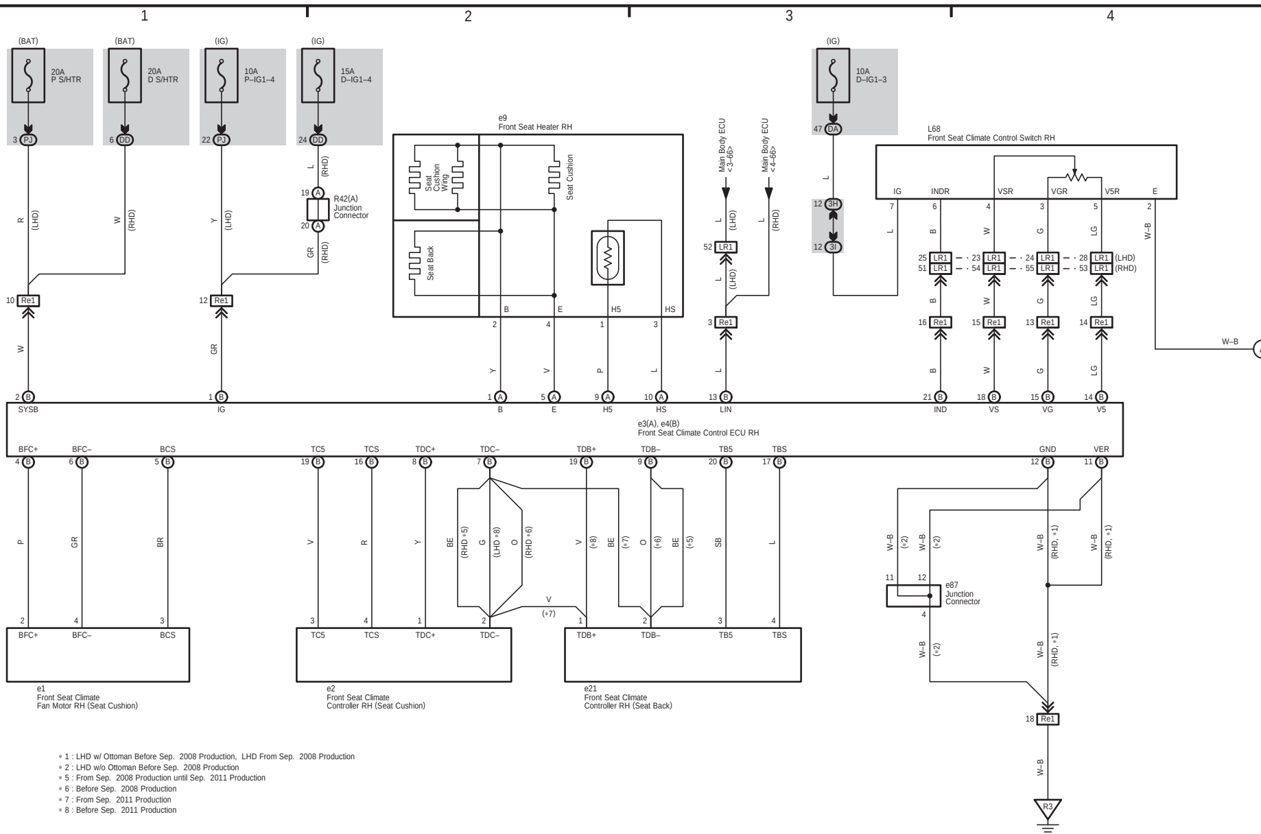
Climate Control Seat (Front LH Seat and Front RH Seat) (Before Sep. 2012 Production)
