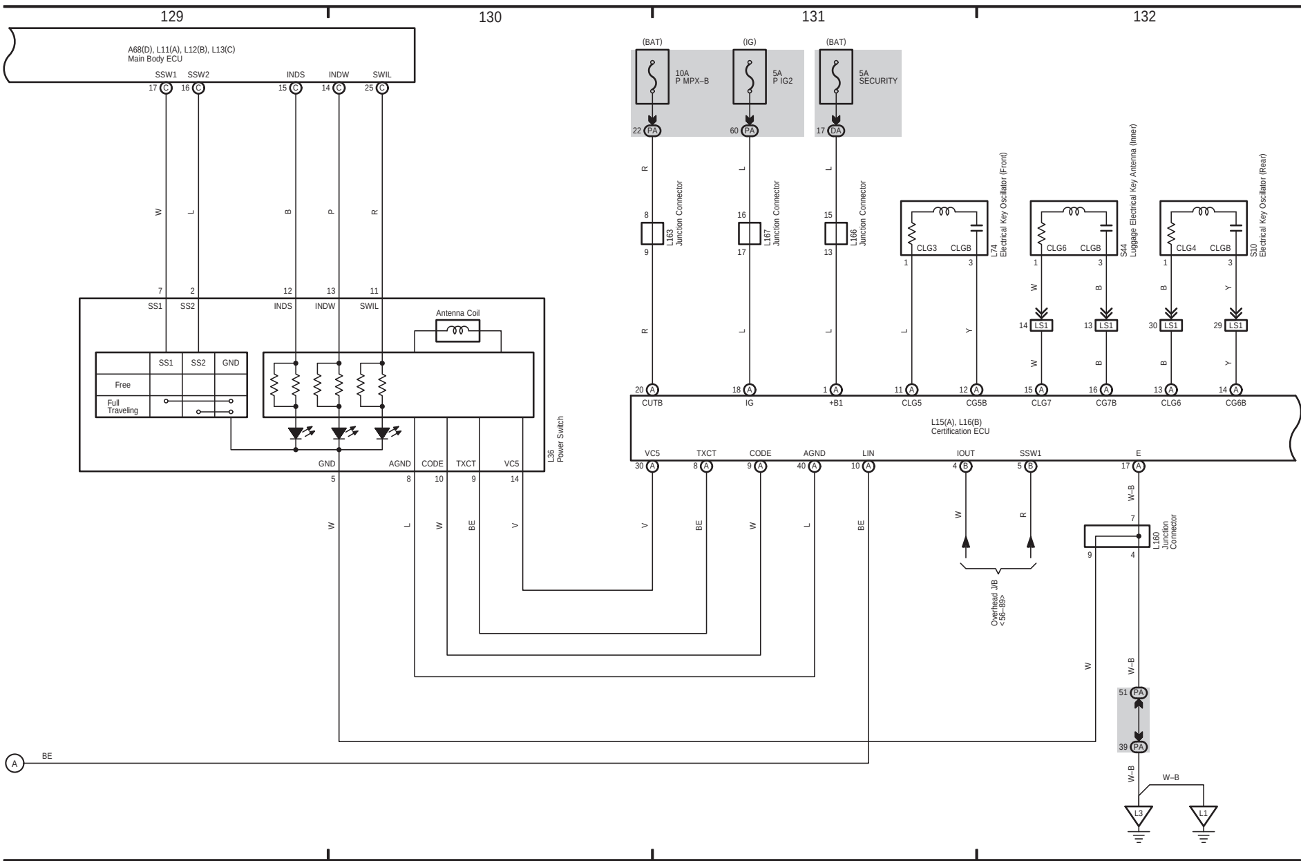
Multiplex Communication System (CAN RHD) (From Sep. 2012 Production)
