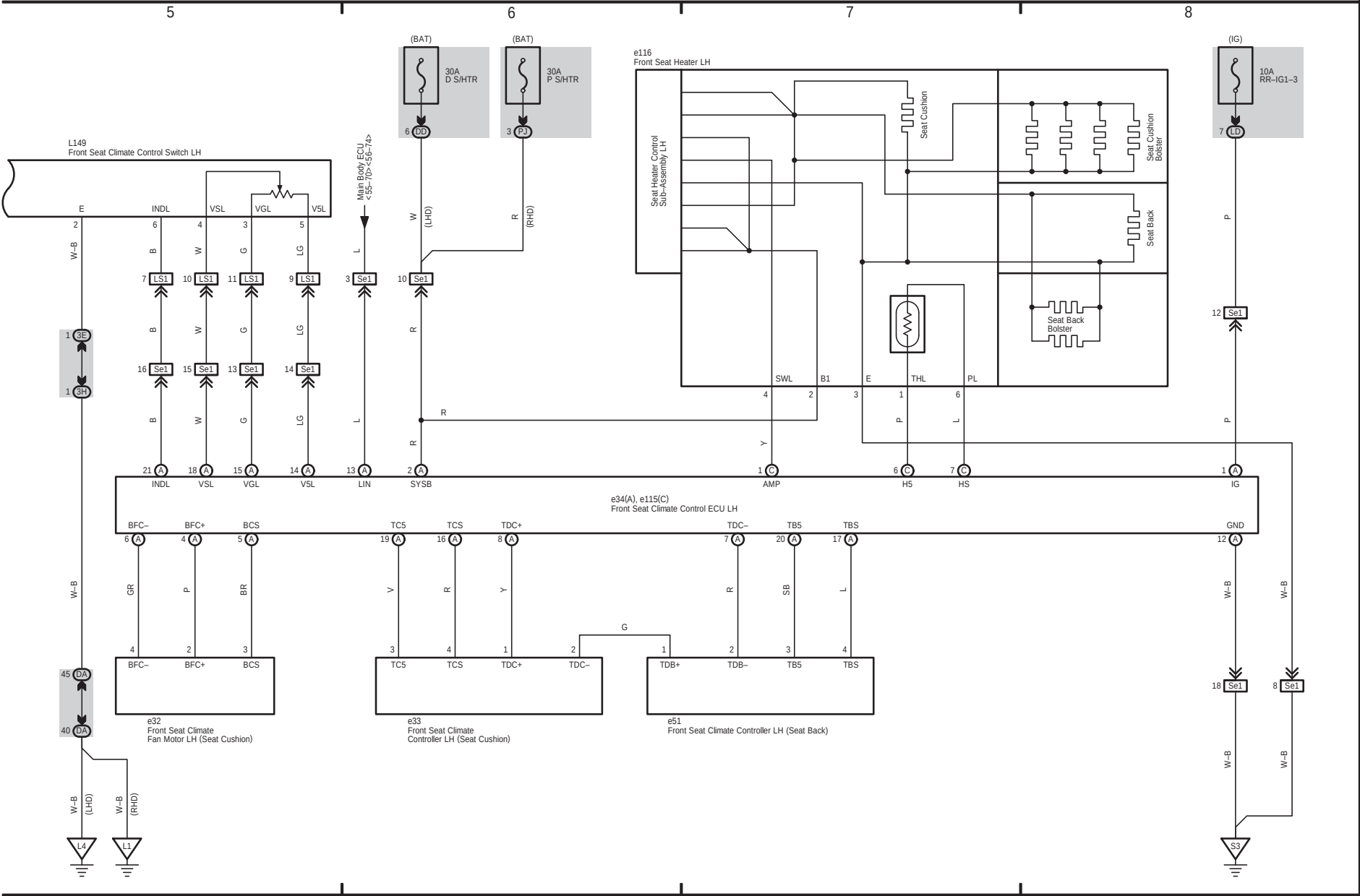
Climate Control Seat (Front LH Seat and Front RH Seat) (From Sep. 2012 Production)
