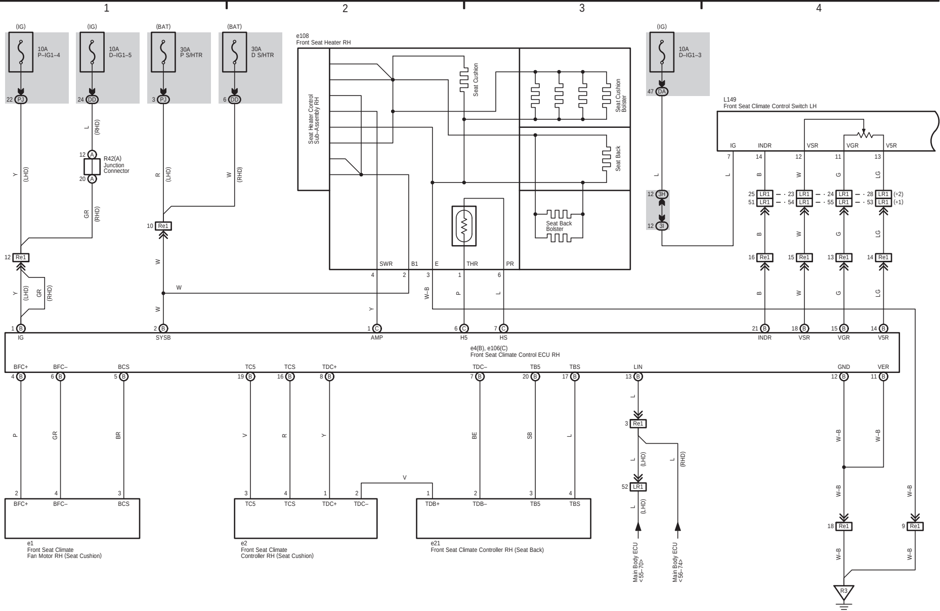
Climate Control Seat (Front LH Seat and Front RH Seat) (From Sep. 2012 Production)
