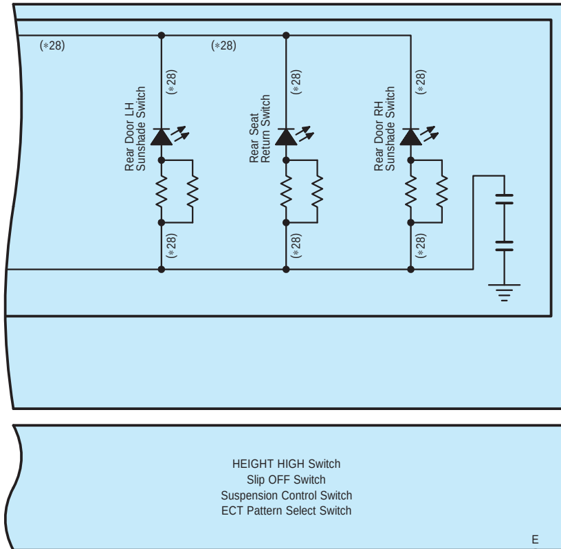
L75(A), z14(C) Console Switch
