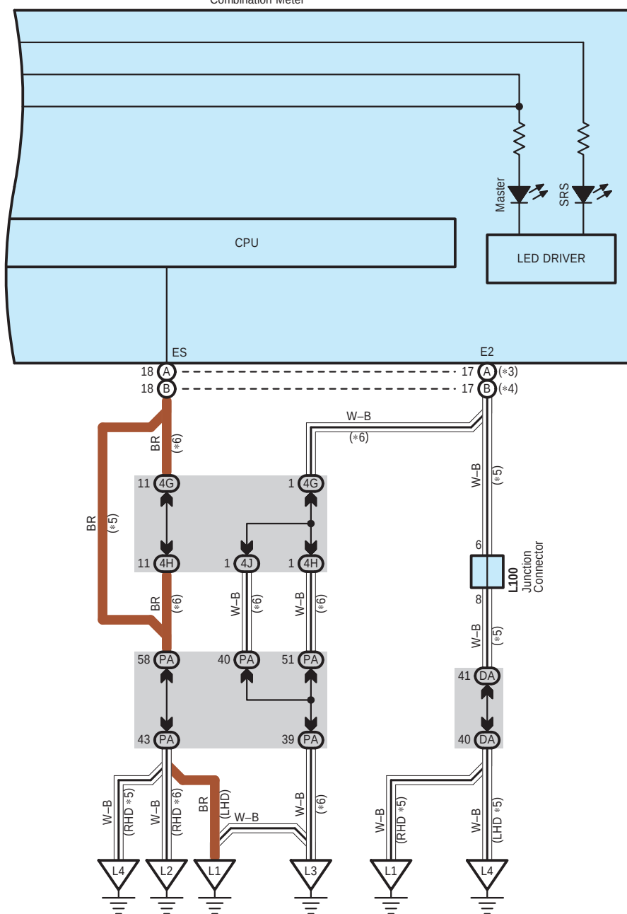
L10(A), (B) Combination Meter
