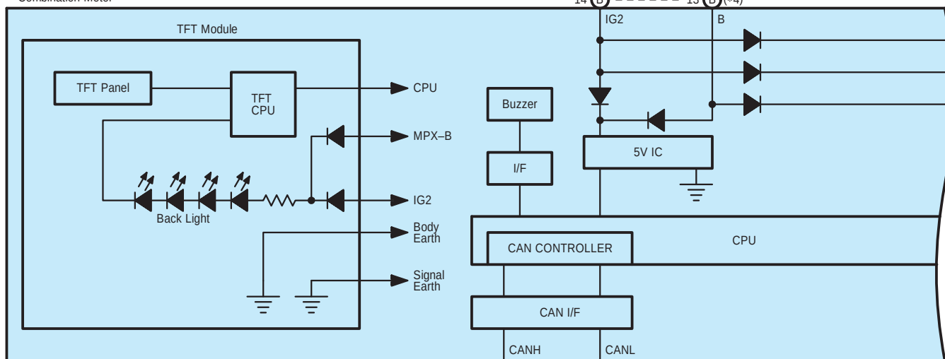
L10(A), (B) Combination Meter
