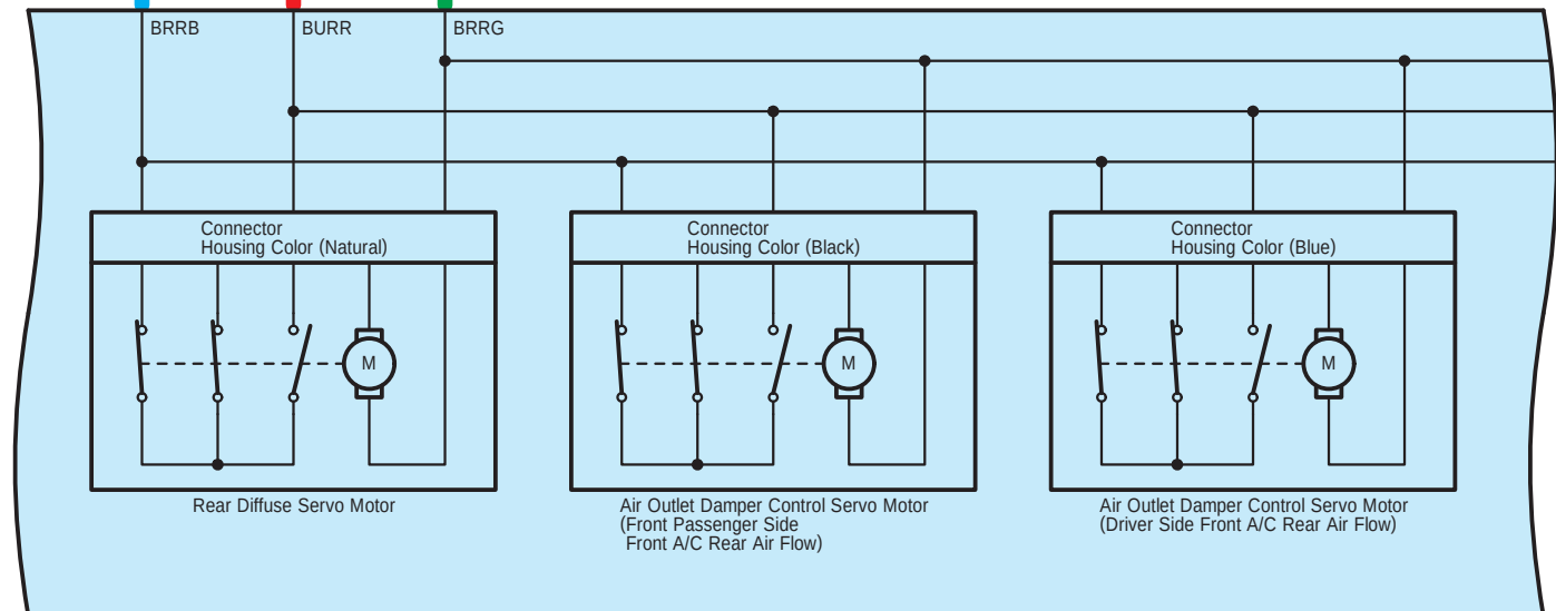
S90 Rear Cooling Unit Assembly
