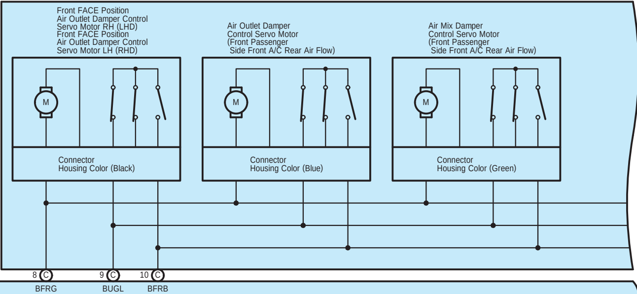
L76(A), L77(B), z1(C) A/C Amplifier
