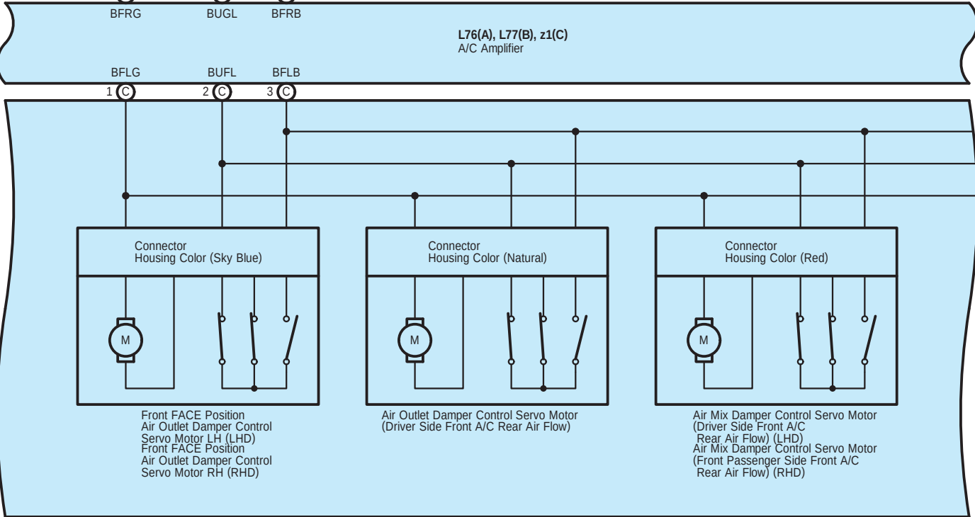
z1(C) A/C Blower Assembly
