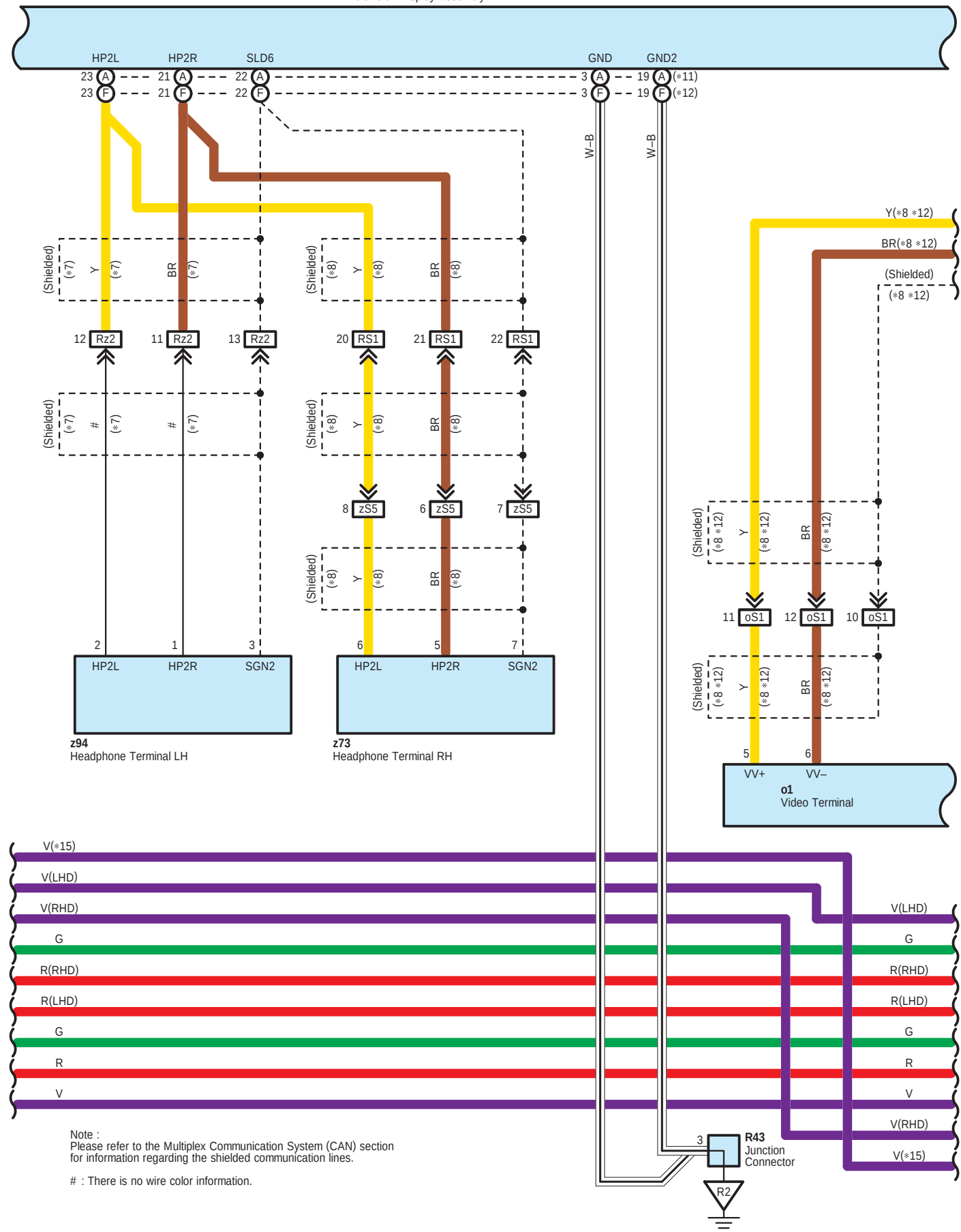
R92(A), R104(B), R105(C), R106(D), R111(E), R112(F) Television Display Assembly
