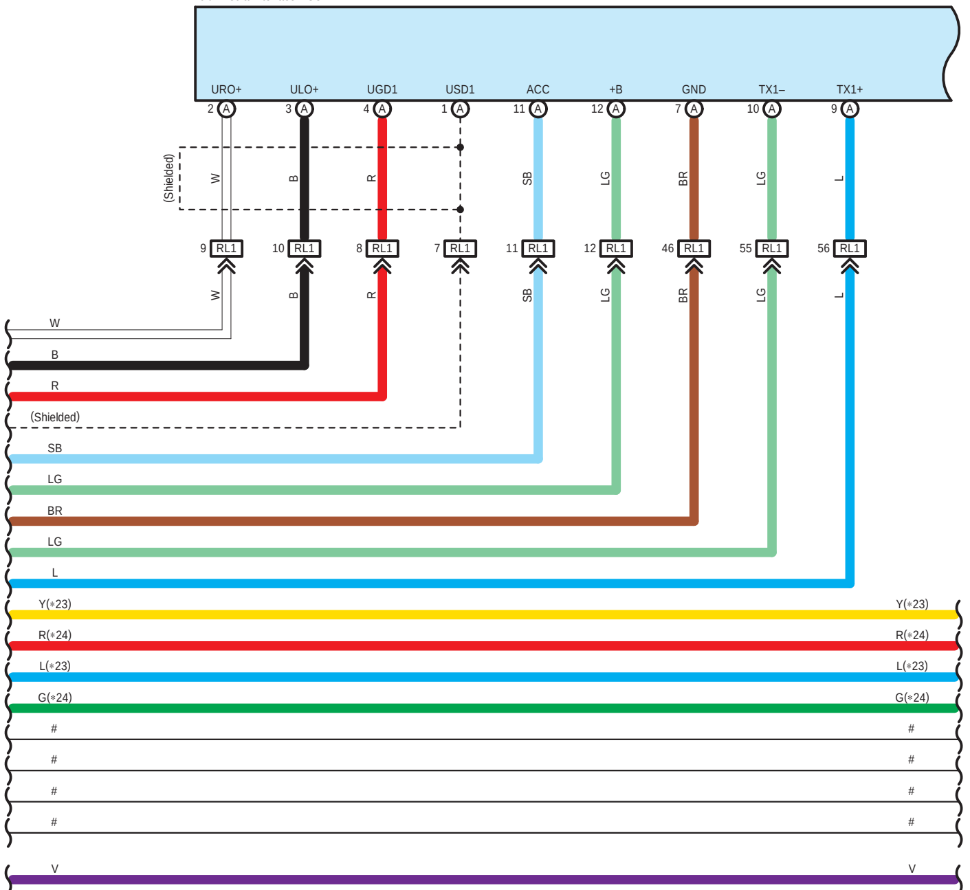
R81(A), R82(B), y1(C) Multi-Media Interface ECU
