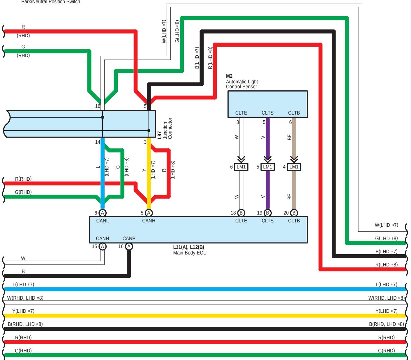
E49 Park/Neutral Position Switch
