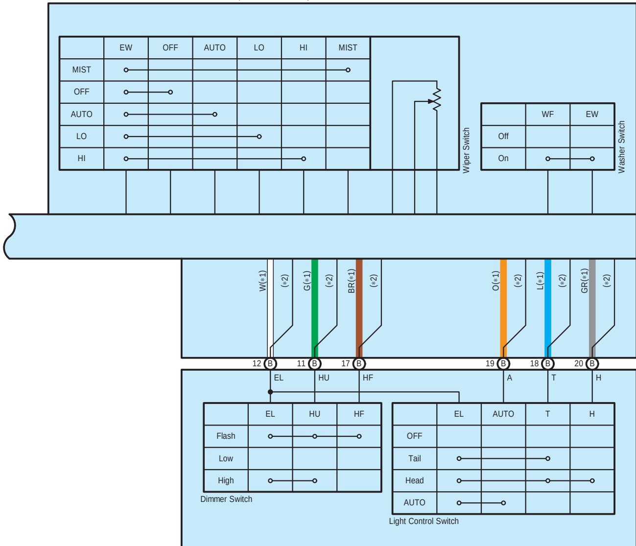
z6(B) Headlight Dimmer Switch Assembly
