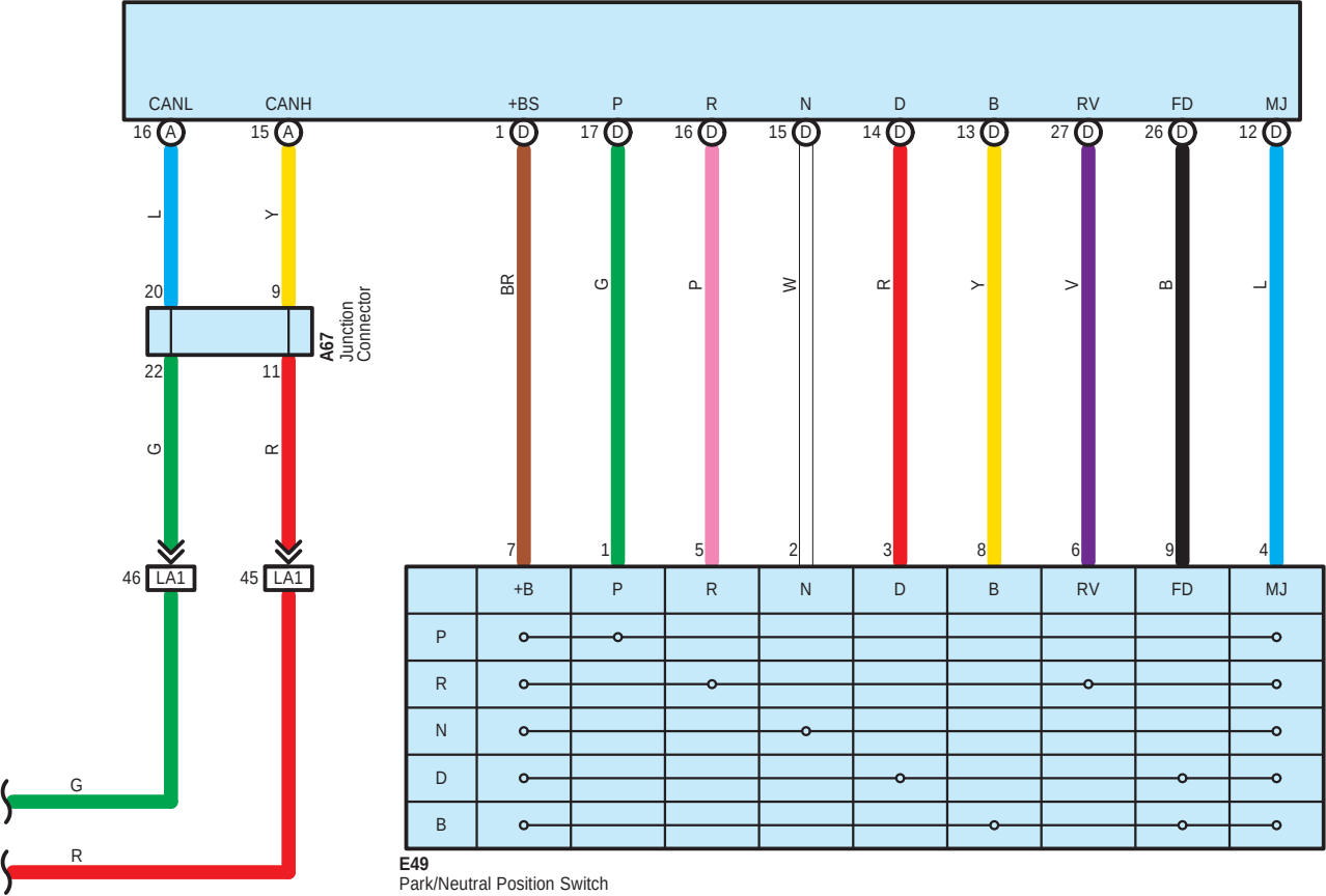
A76(A), E58(D) Hybrid Vehicle Control ECU
