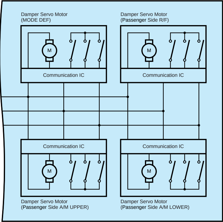
z11(D) Air Conditioning Harness Assembly
