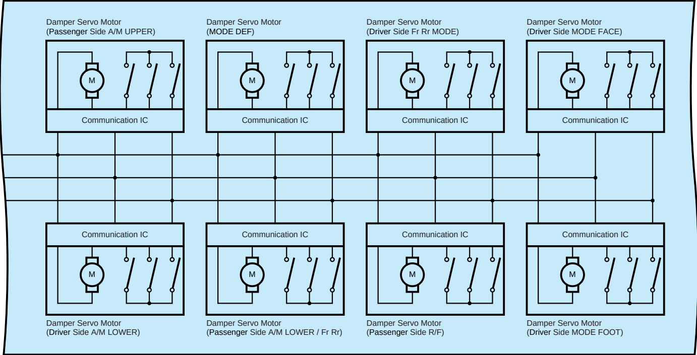
z22(E) Air Conditioning Harness Assembly
