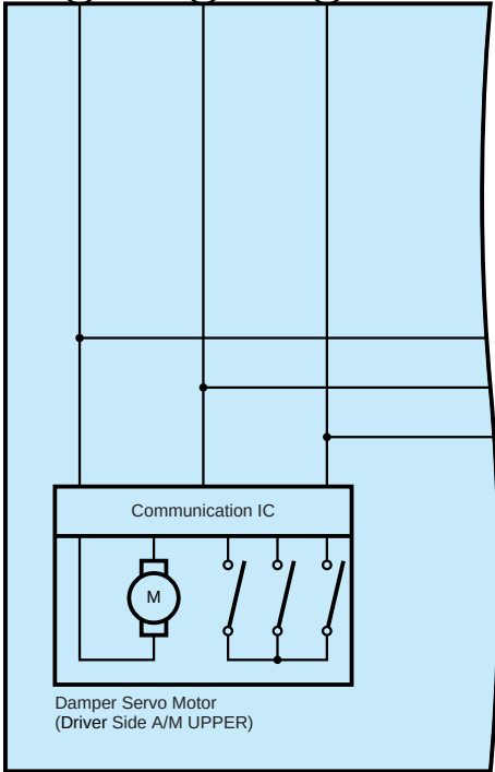
z22(E) Air Conditioning Harness Assembly
