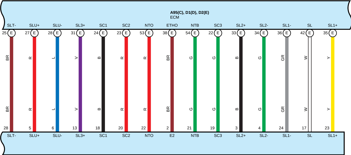
D3 Automatic Transmission Assembly (Transmission Wire)
