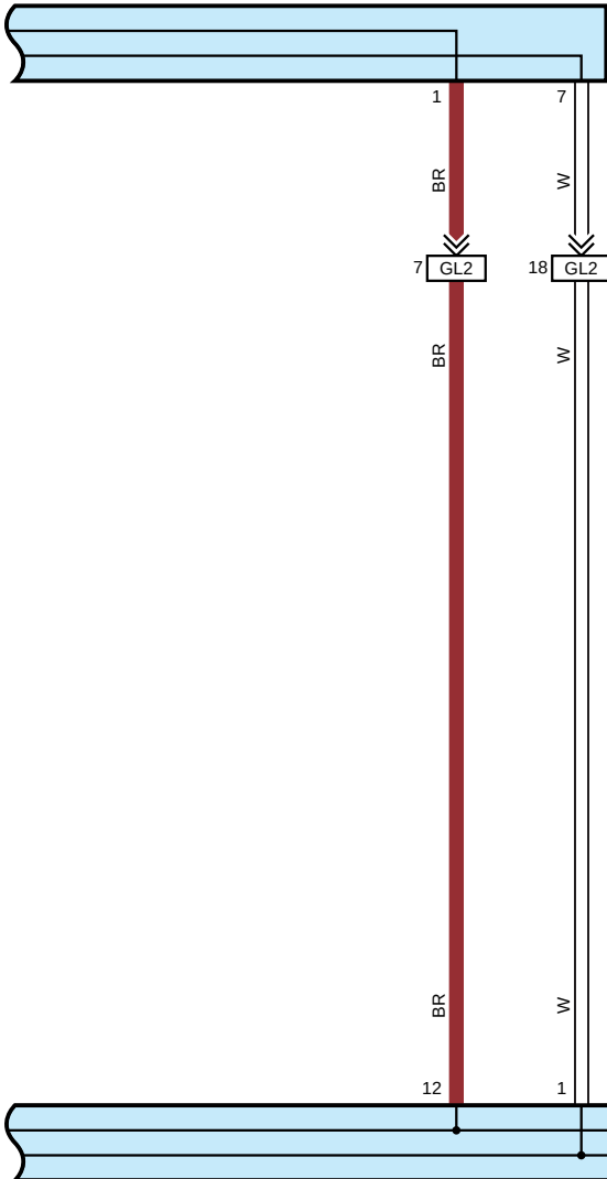
L117 No. 12 CAN Junction Connector
