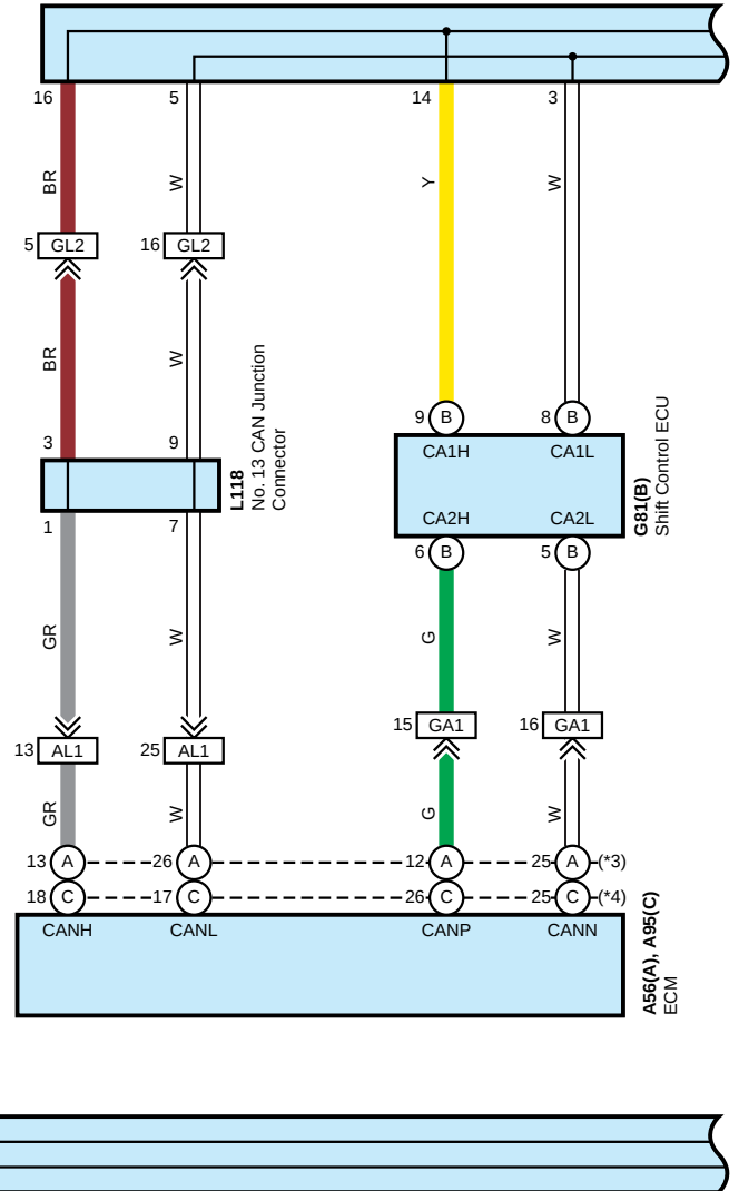
G122 No. 4 CAN Junction Connector
