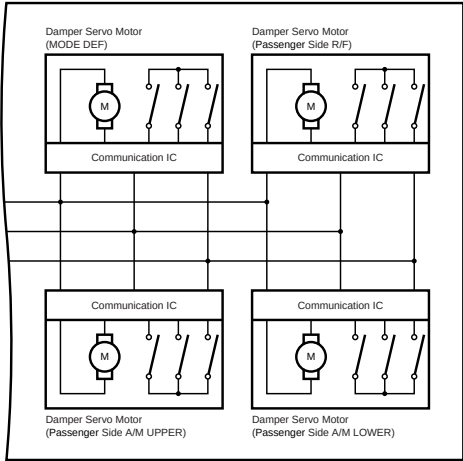
z11(D) Air Conditioning Harness Assembly
