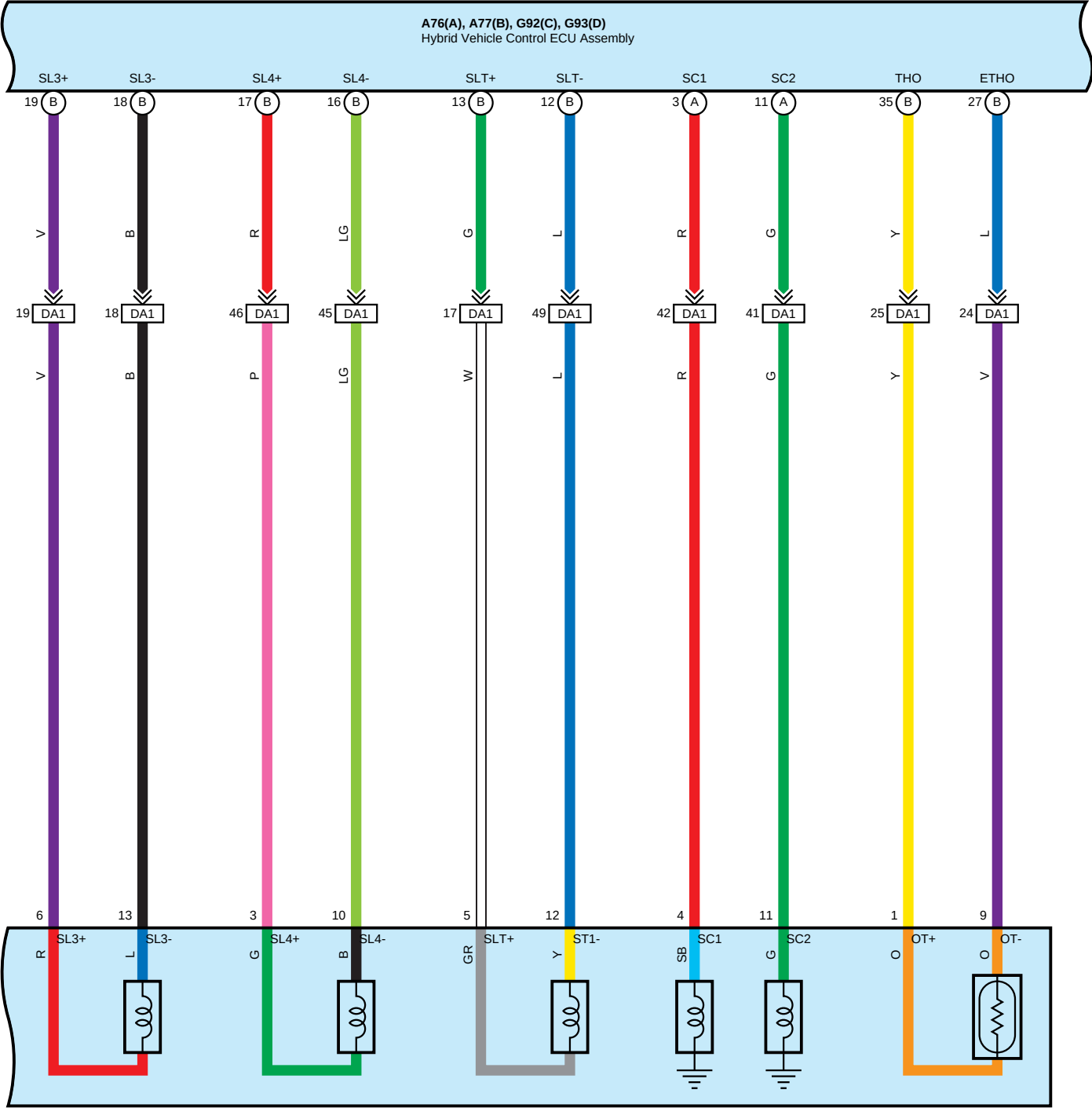
D8 Hybrid Vehicle Transmission Assembly (Transmission Wire)
