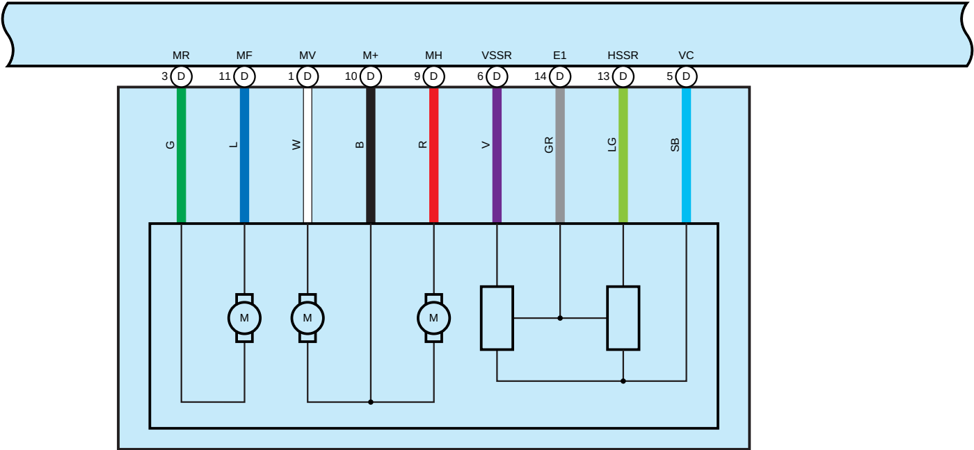
z37(D) Outer Rear View Mirror Assembly RH
