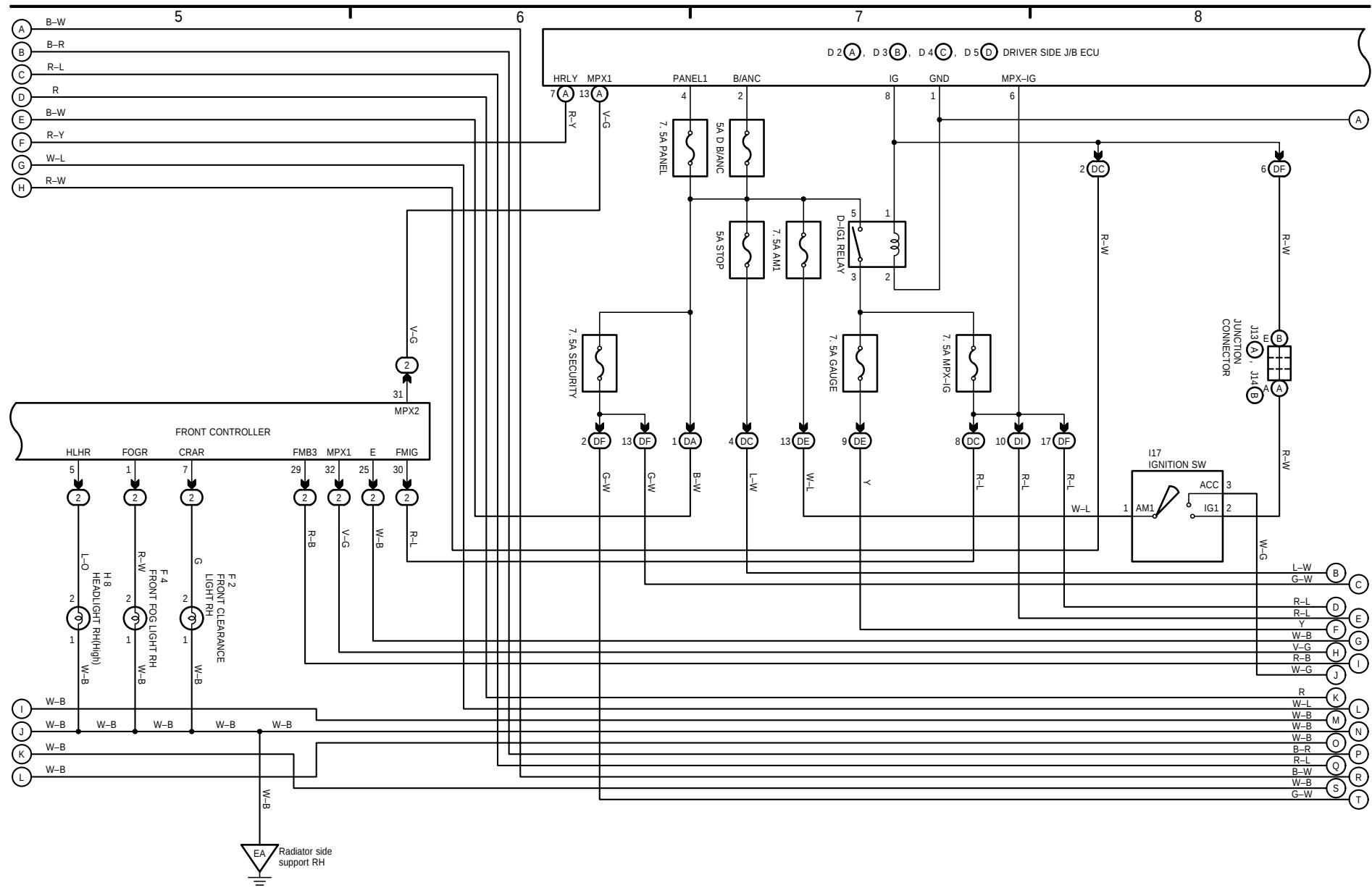
Multiplex Communication System (J/B ECU)
