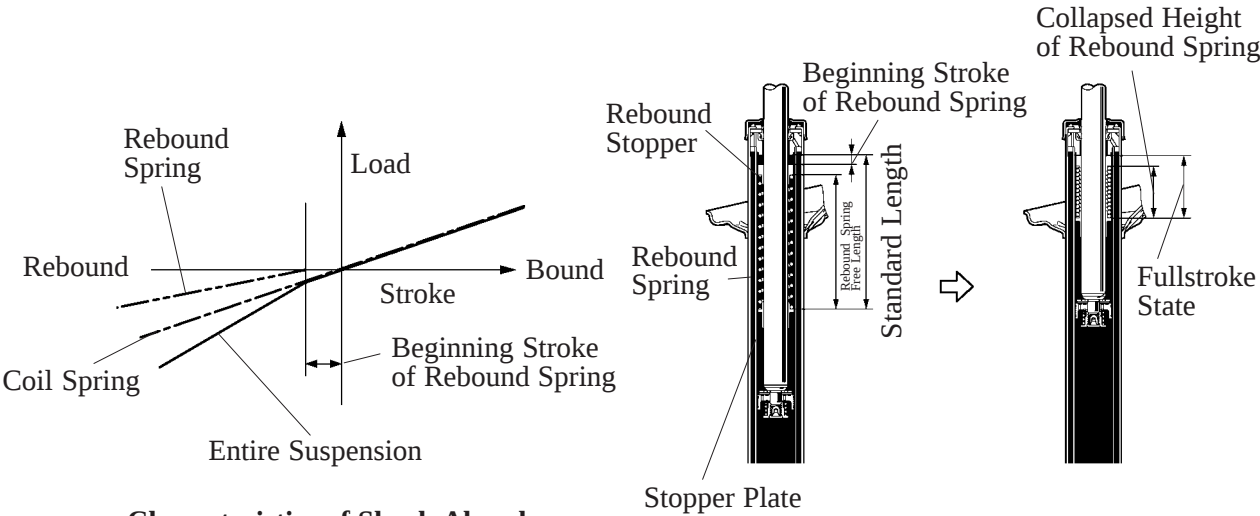
Characteristics of Shock Absorber with Built-in Rebound Spring
