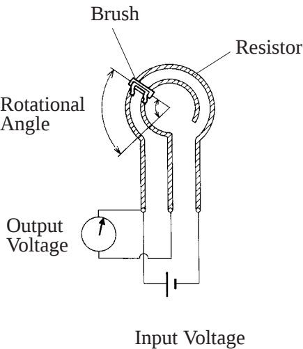
Diagram of the Principle
