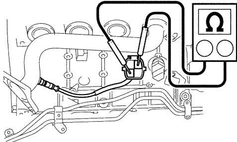
Bank 1 sensor 2
