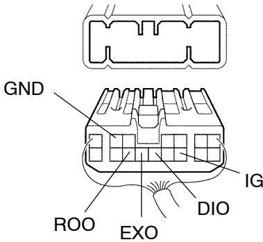
Rear Air Conditioning Amplifier Connector Wire Harness View:
