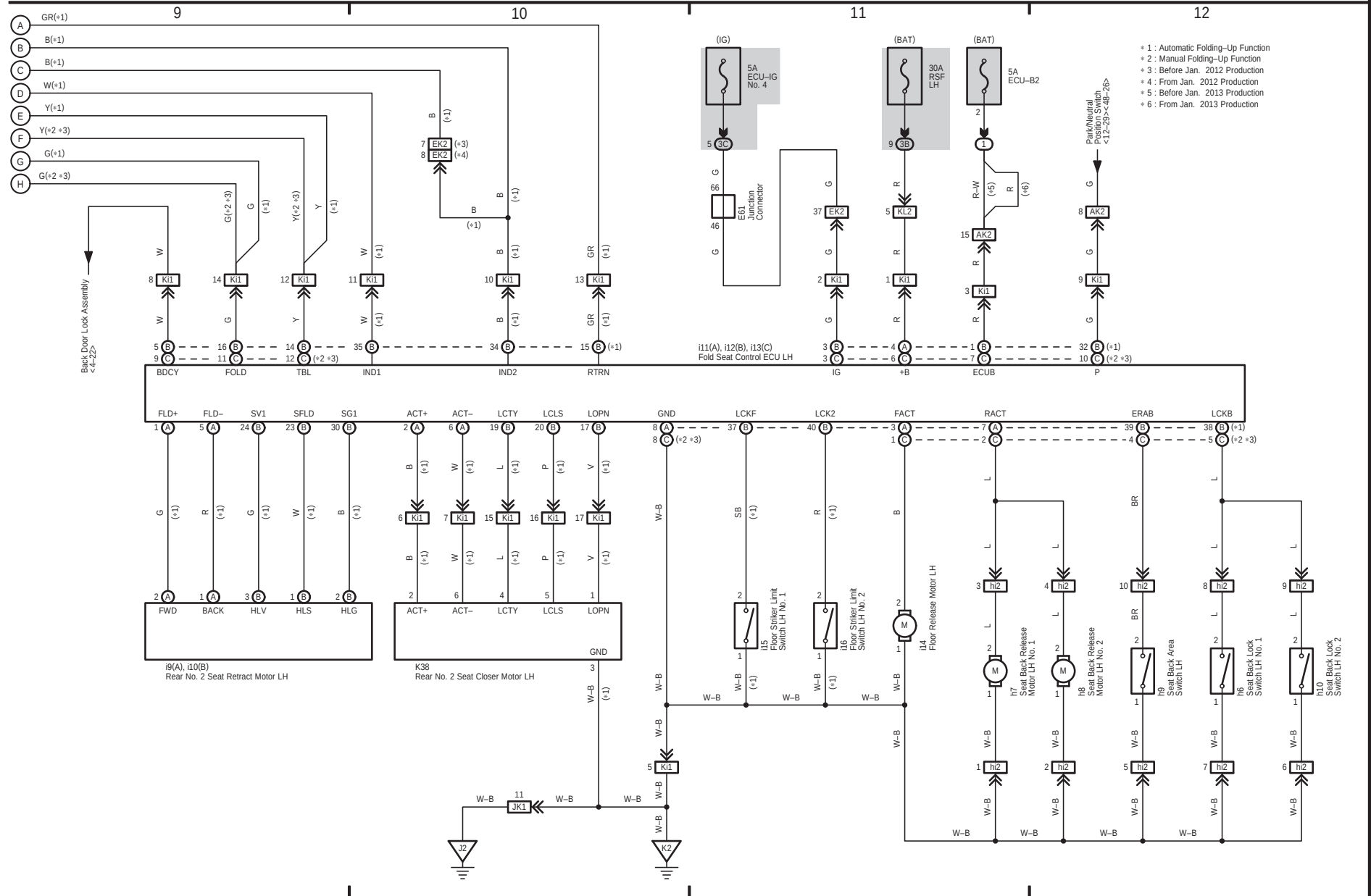
Rear Power Seat Control System (for Rear No. 2 Seat with Folding-Up Function) (Before Sep. 2015 Production)
