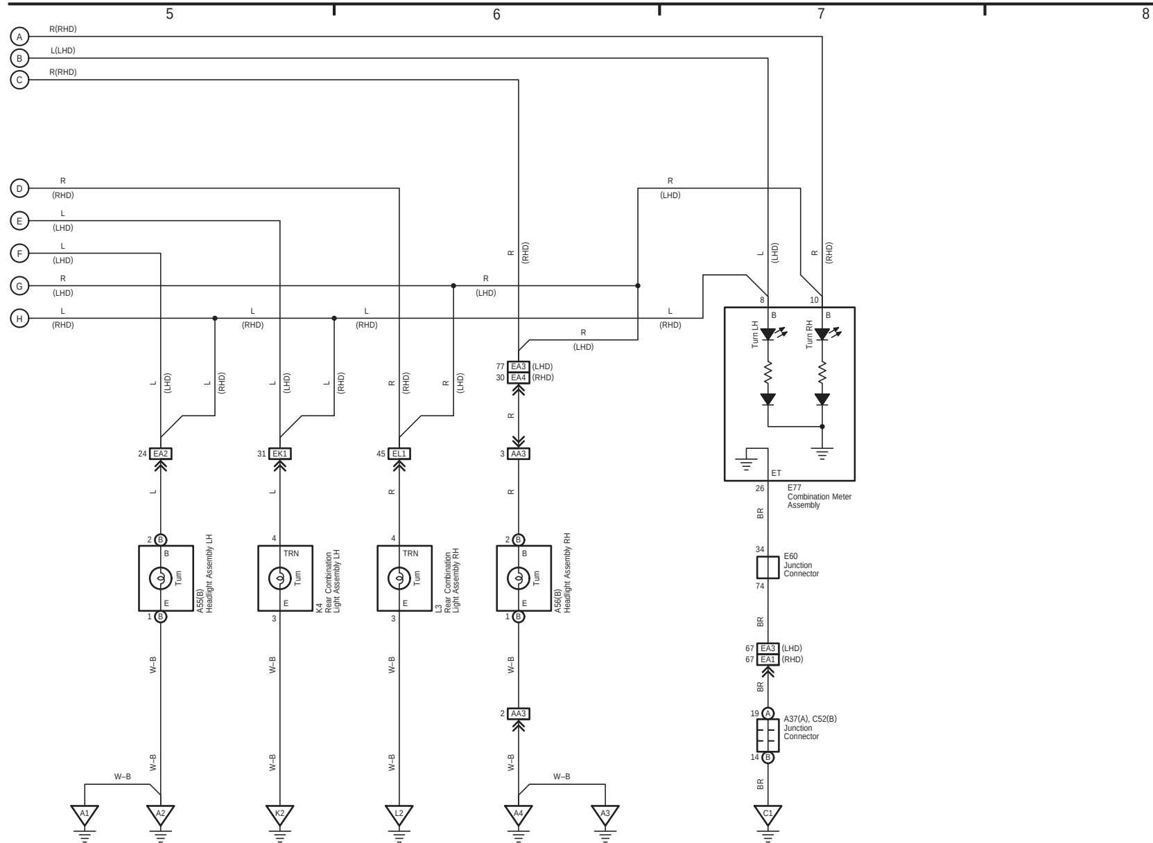
Turn Signal and Hazard Warning Light (From Jan. 2012 Production until Sep. 2015 Production)
