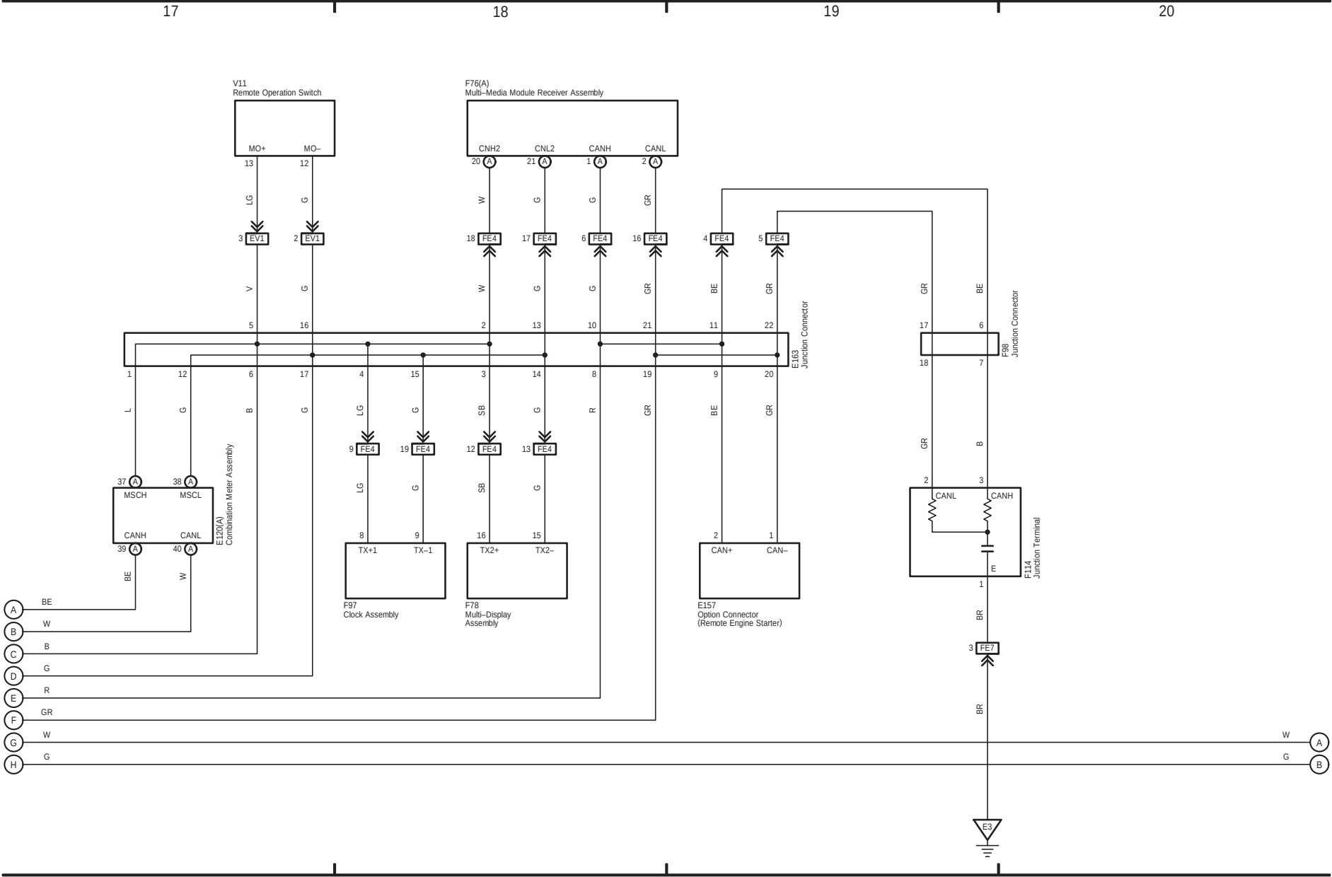
Multiplex Communication System (CAN) (RHD) (From Sep. 2015 Production)
