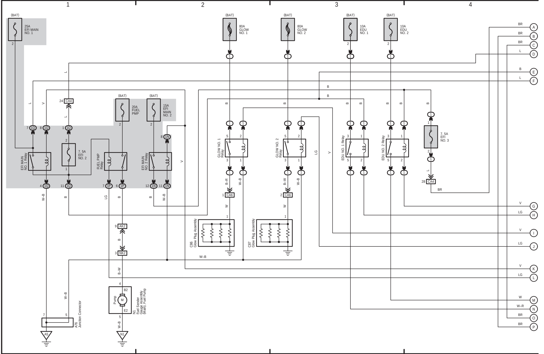
Engine Control (1VD-FTV w/o DPF) (From Sep. 2015 Production)
