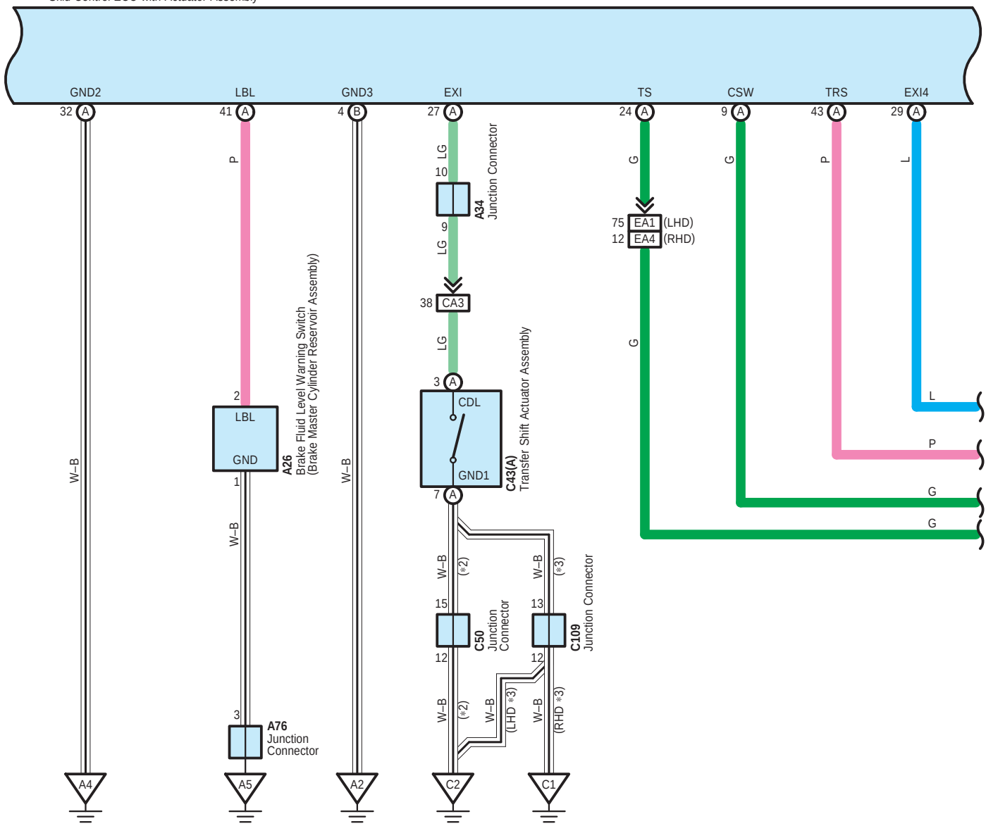
A24(A), A25(B) Skid Control ECU with Actuator Assembly
