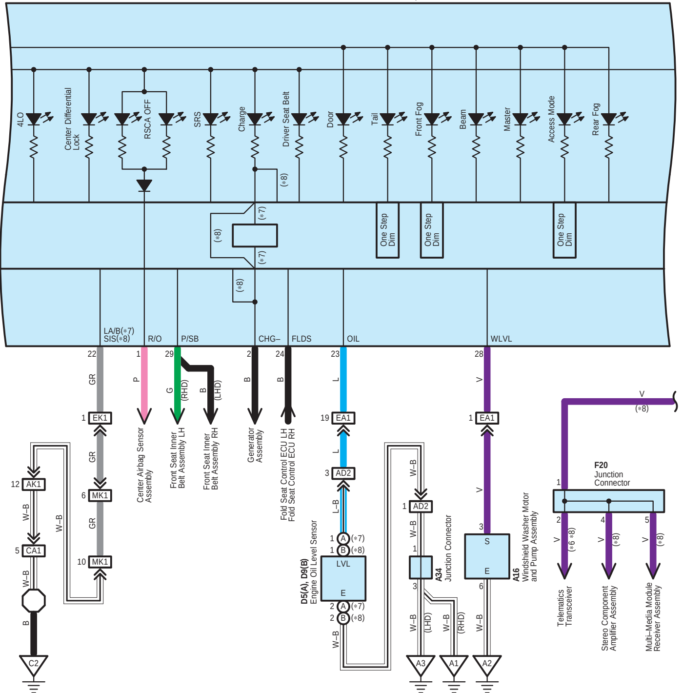
E77 Combination Meter Assembly
