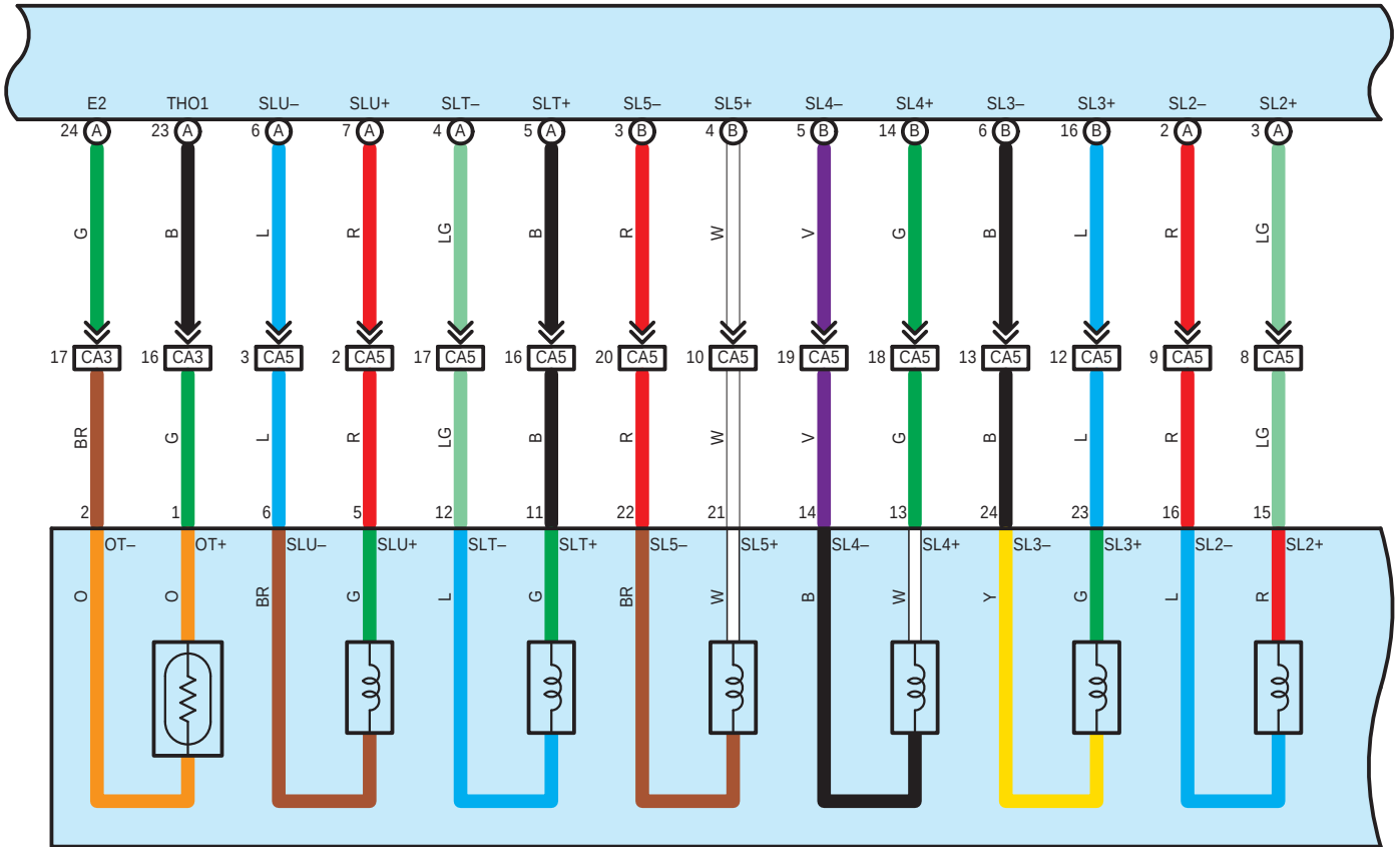
C67 Electronically Controlled Transmission Solenoid
