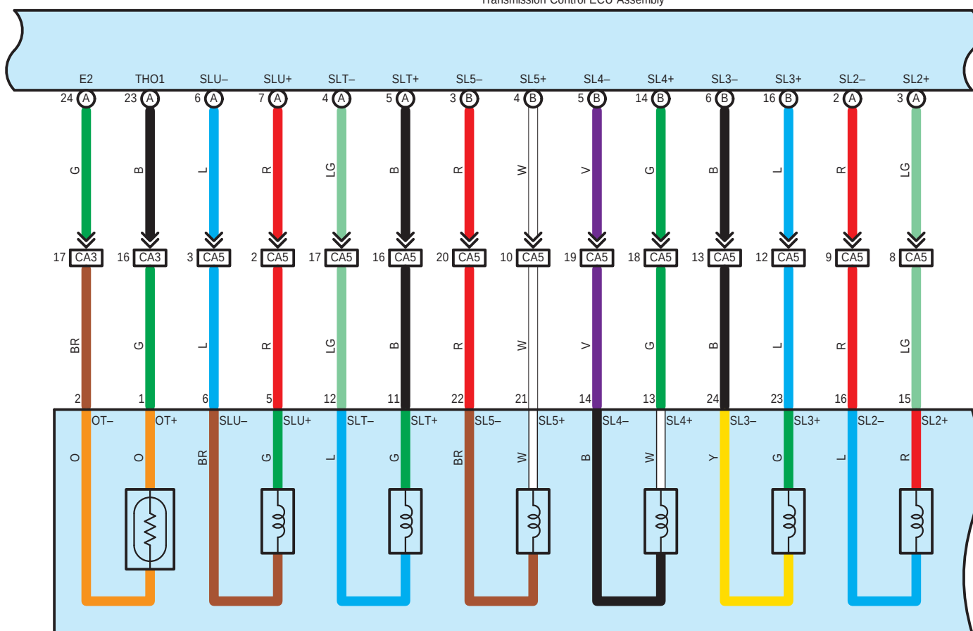
C67 Electronically Controlled Transmission Solenoid
